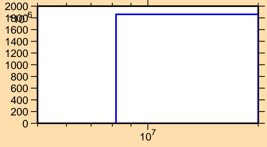
\sigma vs. E for ^{45}\text{Sc}(n,n\alpha)
