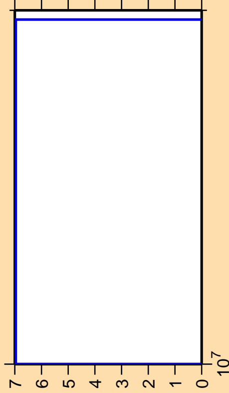
\Delta\sigma/\sigma vs. E for ^{46}\text{Sc}(n,nt)
