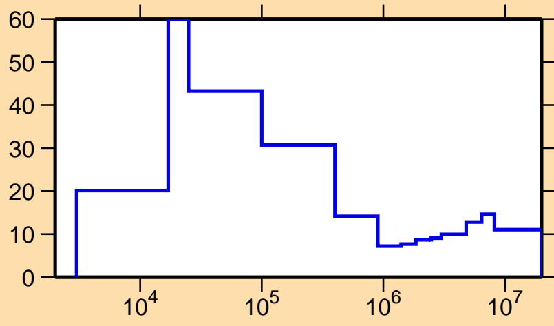
\Delta\sigma/\sigma vs. E for ^{46}\text{Sc}(n,el.)
