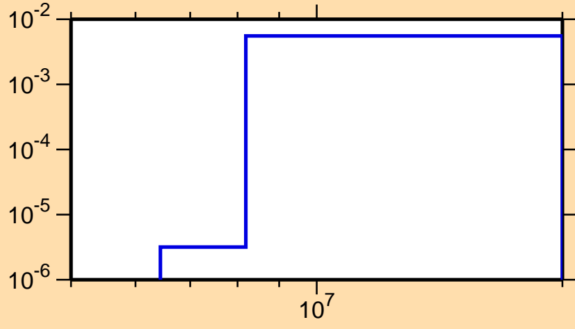
\sigma vs. E for ^{46}\text{Sc}(n,d)
