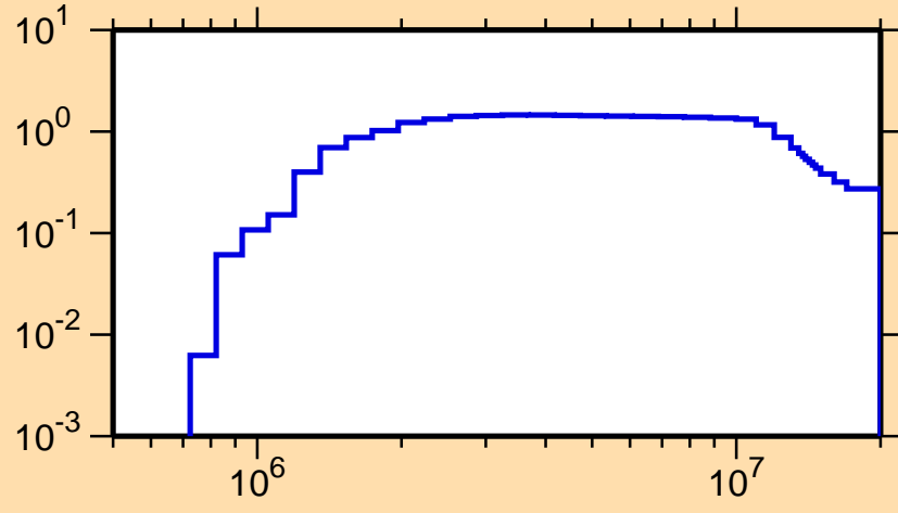
\sigma vs. E for ^{47}\text{Sc}(n,\text{inel.})
