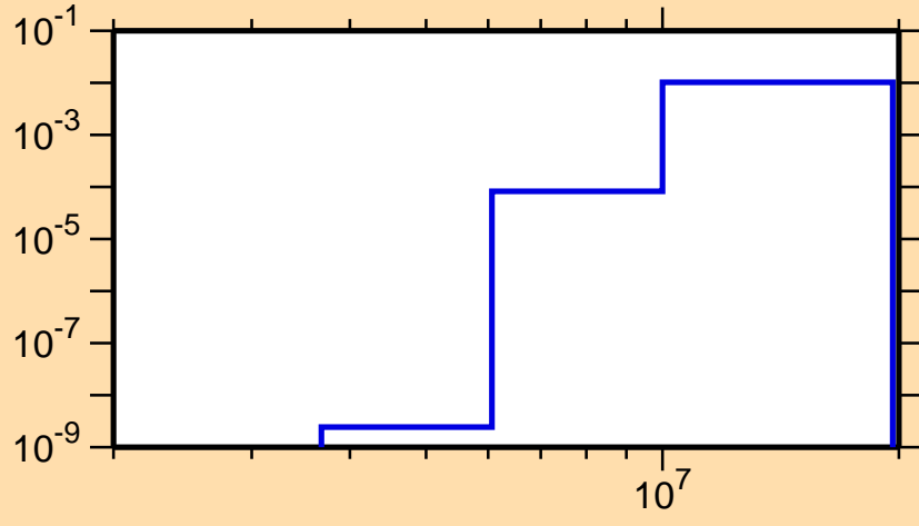
\sigma vs. E for ^{47}\text{Sc}(n,\alpha)
