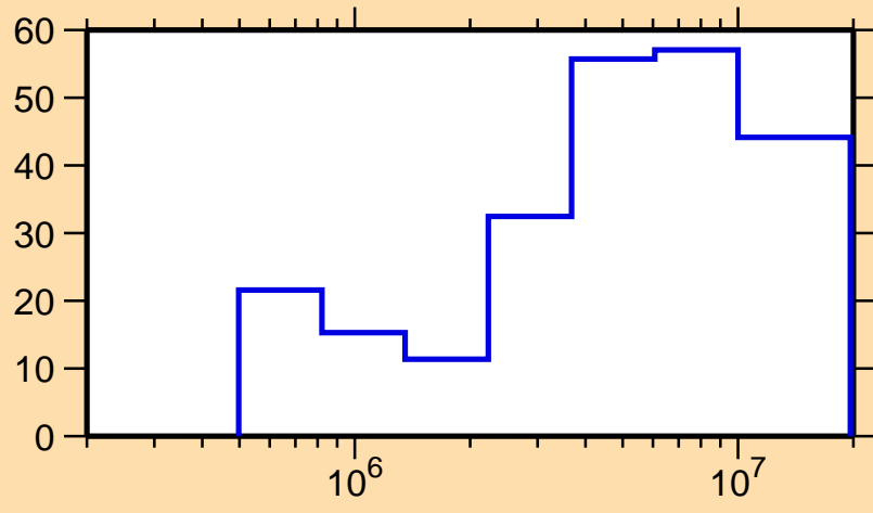
\Delta\sigma/\sigma vs. E for ^{47}\text{Sc}(n,n_1)
