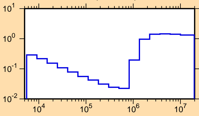
\sigma vs. E for ^{47}\text{Sc}(n,\text{nonel.})
