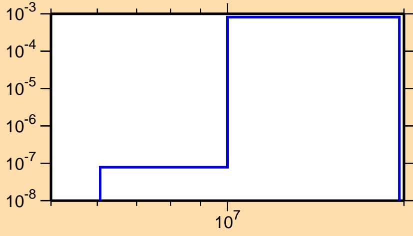
\sigma vs. E for ^{49}\text{Sc}(n,\alpha)
