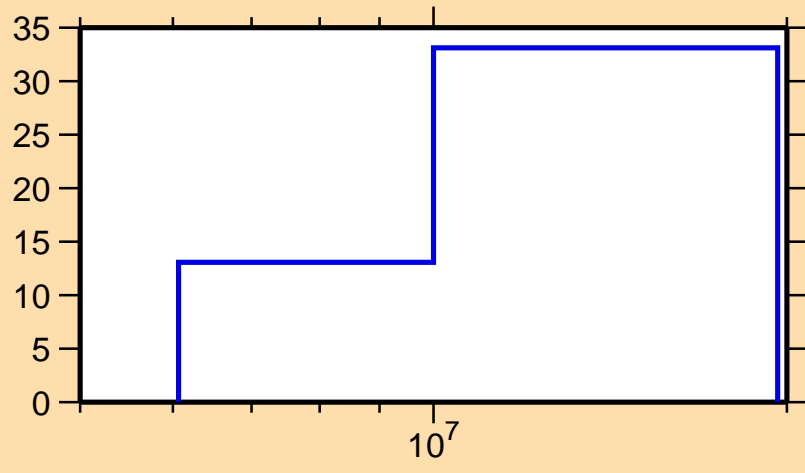
\Delta\sigma/\sigma vs. E for ^{49}\text{Sc}(n,ncont.)
