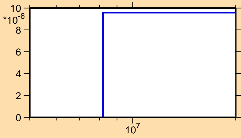
\sigma vs. E for ^{49}\text{Sc}(n,t)
