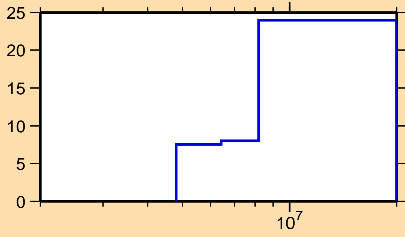
\Delta\sigma/\sigma vs. E for ^{49}\text{Sc}(n,\text{inel.})
