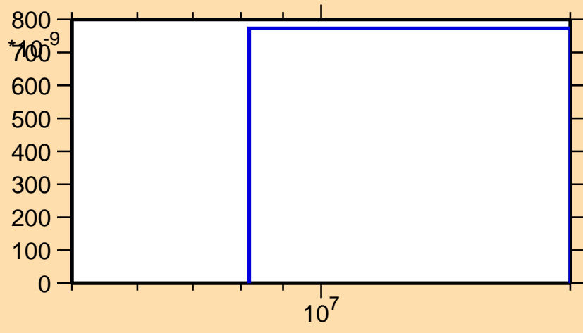
\sigma vs. E for ^{49}\text{Sc}(n,3n)
