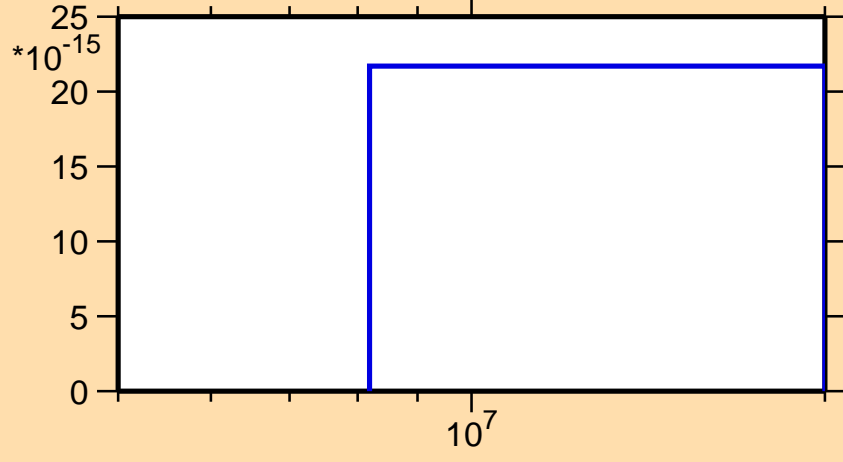
\sigma vs. E for ^{49}\text{Sc}(n,nt)
