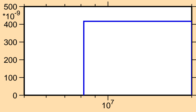
\sigma vs. E for ^{49}\text{Sc}(n,n\alpha)
