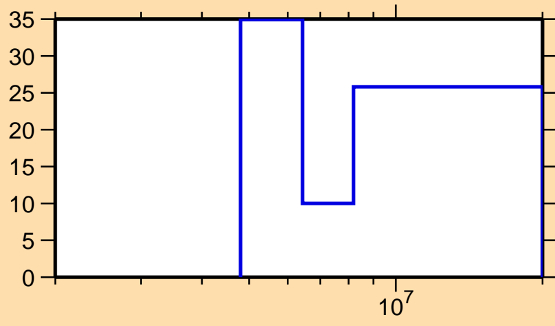
\Delta\sigma/\sigma vs. E for ^{49}\text{Sc}(n,n\text{cont.})
