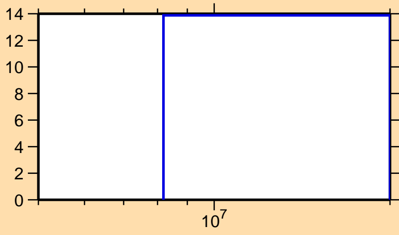
\Delta\sigma/\sigma vs. E for ^{49}\text{Sc}(n,\text{el.})
