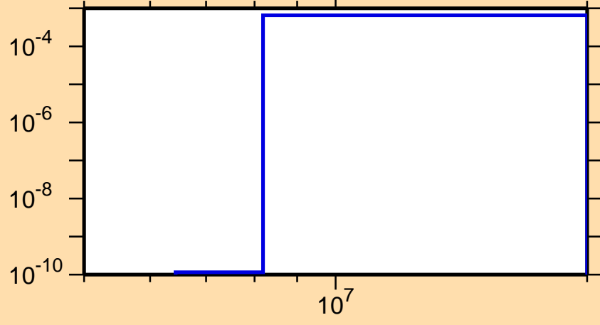
\sigma vs. E for ^{49}\text{Sc}(n,\alpha)
