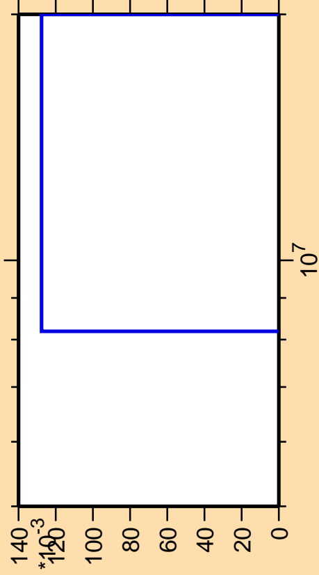
\Delta\sigma/\sigma vs. E for ^{49}\text{Sc}(n,nt)
