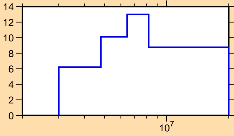
\Delta\sigma/\sigma vs. E for ^{49}\text{Sc}(n,\text{tot.})
