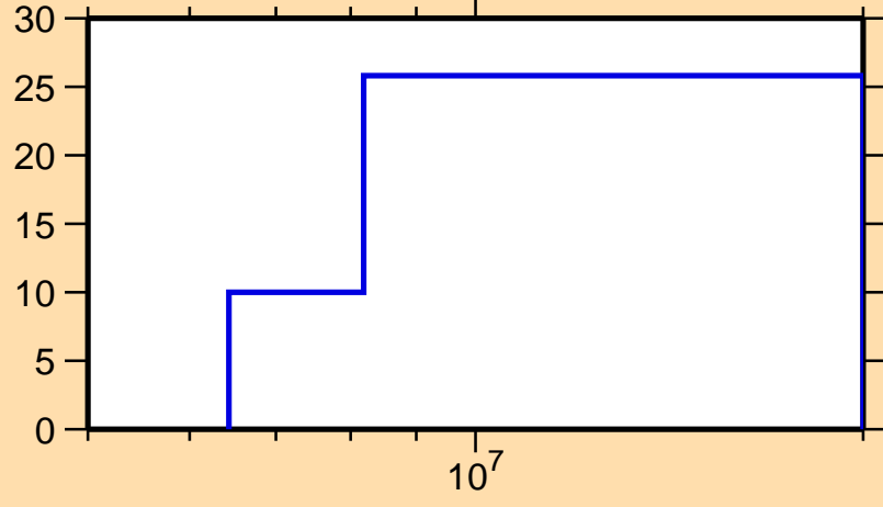
\Delta\sigma/\sigma vs. E for ^{49}\text{Sc}(n,n\text{cont.})
