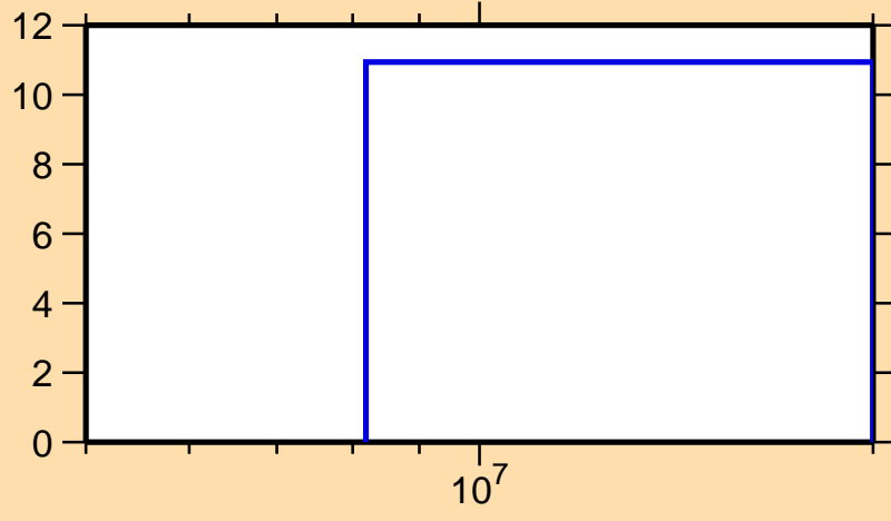
\Delta\sigma/\sigma vs. E for ^{49}\text{Sc}(n,2n)
