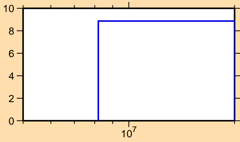
\Delta\sigma/\sigma vs. E for ^{49}\text{Sc}(n,\text{nonel.})
