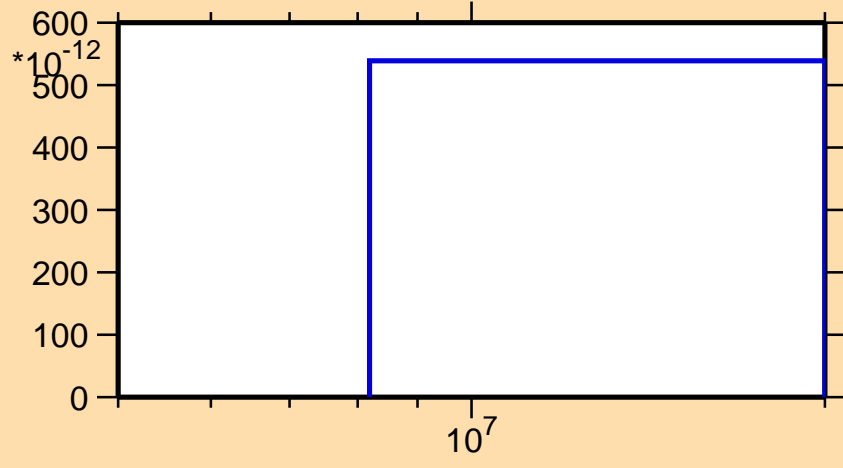
\sigma vs. E for ^{49}\text{Sc}(n,\text{nd})
