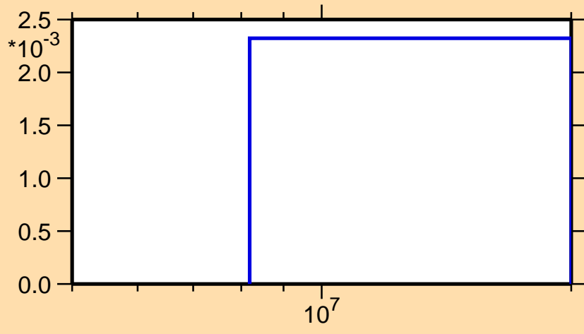
\sigma vs. E for ^{49}\text{Sc}(n,np)
