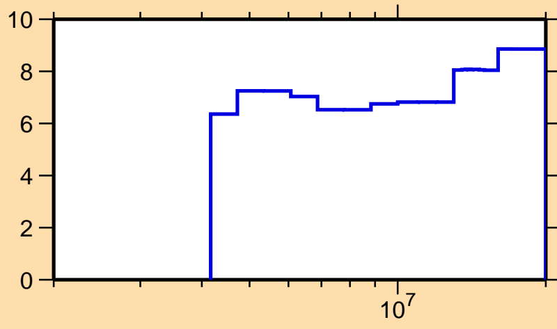
\Delta\sigma/\sigma vs. E for ^{50}\text{Sc}(n,\text{nonel.})
