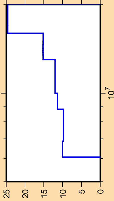
\Delta\sigma/\sigma vs. E for ^{50}\text{Sc}(n,2n)
