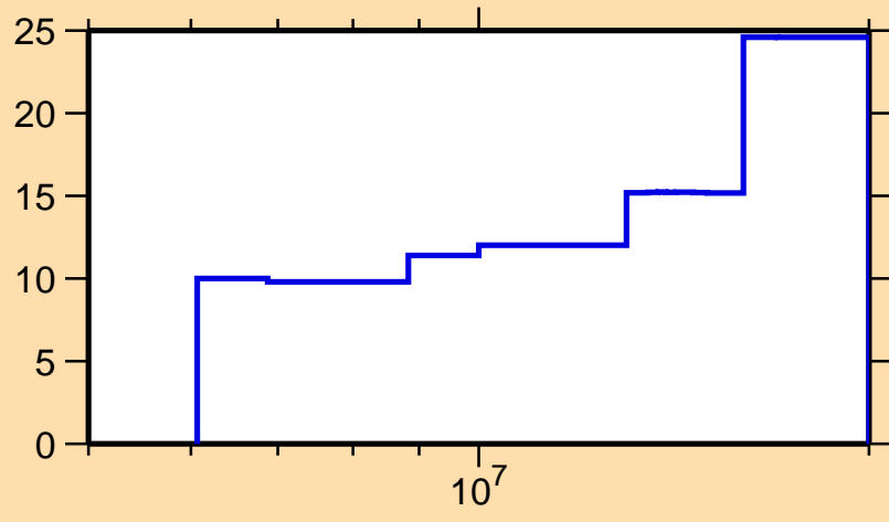
\Delta\sigma/\sigma vs. E for ^{50}\text{Sc}(n,2n)
