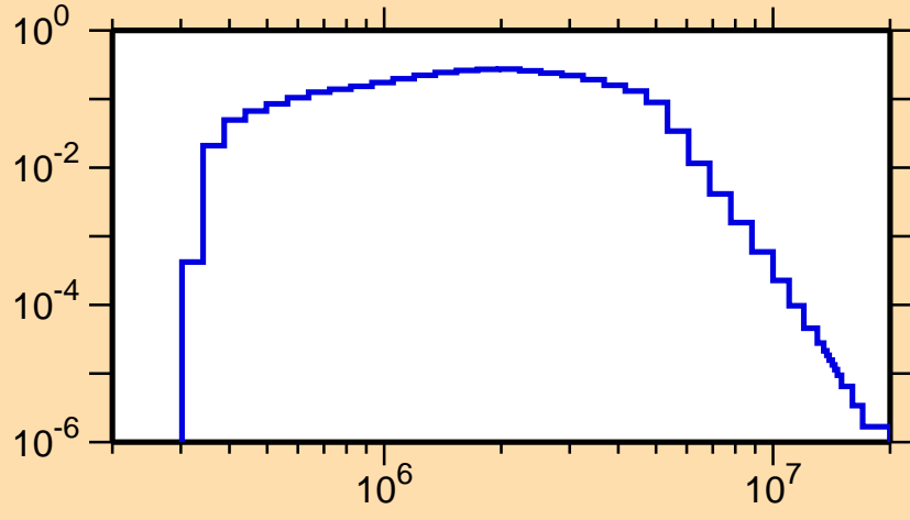
\sigma vs. E for ^{50}\text{Sc}(n,n_2)
