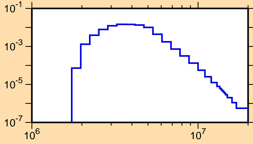
\sigma vs. E for ^{50}\text{Sc}(n,n_4)
