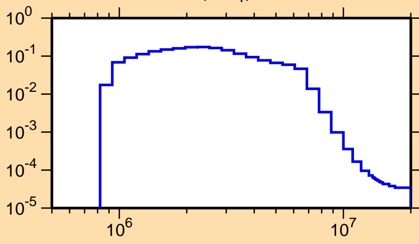
\sigma vs. E for ^{51}\text{Sc}(n,n_1)
