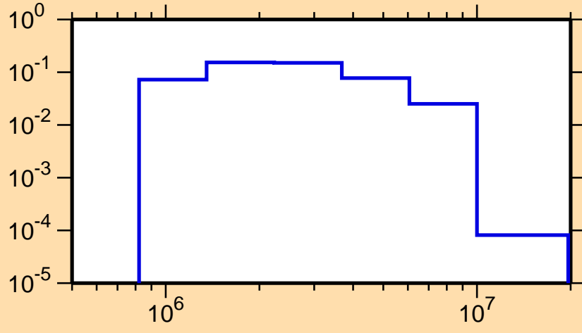
\sigma vs. E for ^{51}\text{Sc}(n,n_1)
