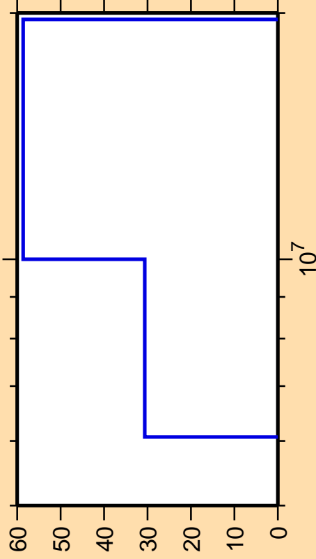
\Delta\sigma/\sigma vs. E for ^{51}\text{Sc}(n,p)
