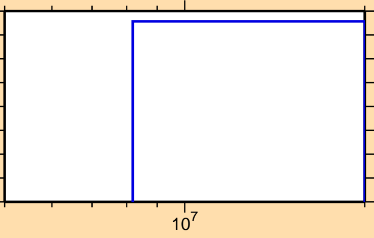
\sigma vs. E for ^{51}\text{Sc}(n,3n)
