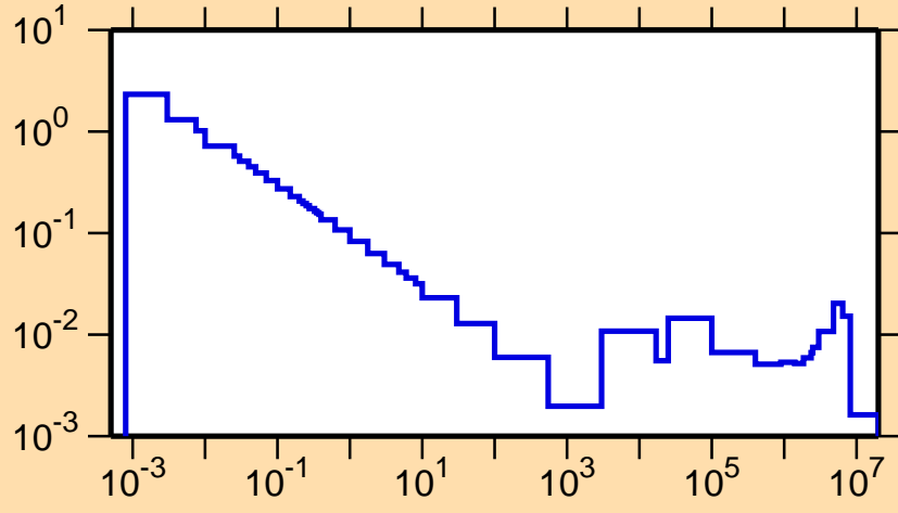
\sigma vs. E for ^{51}\text{Sc}(n,\gamma)
