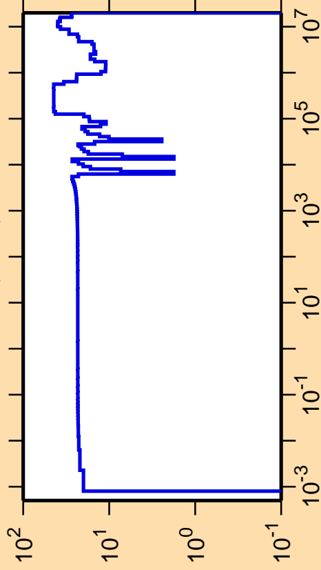
\Delta\sigma/\sigma vs. E for ^{52}\text{Sc}(n,\text{el.})
