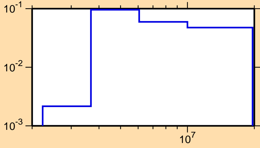
\sigma vs. E for ^{52}\text{Sc}(n,n_4)
