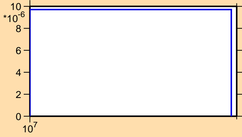
\sigma vs. E for ^{52}\text{Sc}(n,np)
