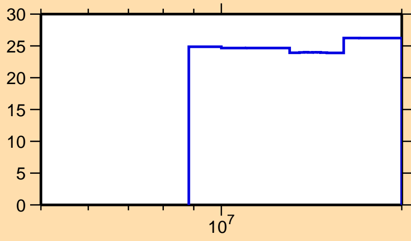
\Delta\sigma/\sigma vs. E for ^{53}\text{Sc}(n,\text{nonel.})
