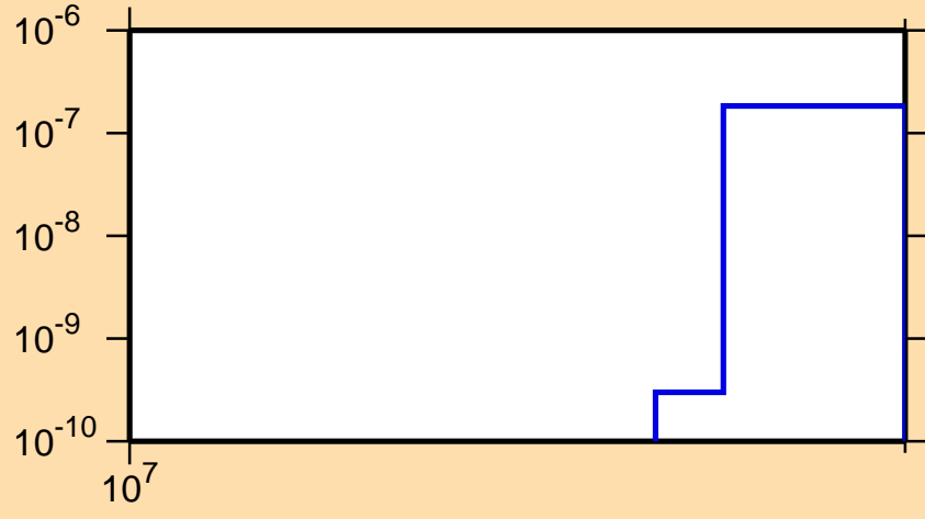
\sigma vs. E for ^{53}\text{Sc}(n,\text{nd})
