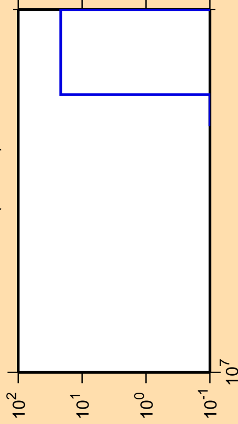
\Delta\sigma/\sigma vs. E for ^{53}\text{Sc}(n,2n\alpha)
