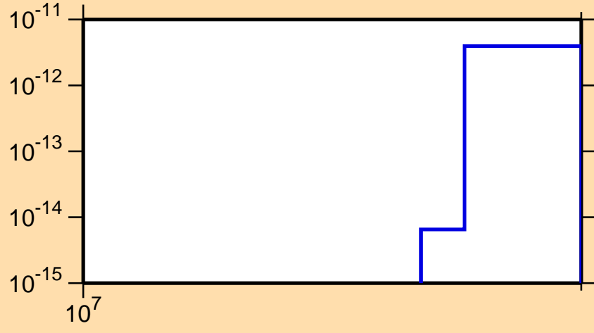
\sigma vs. E for ^{53}\text{Sc}(n,2n\alpha)
