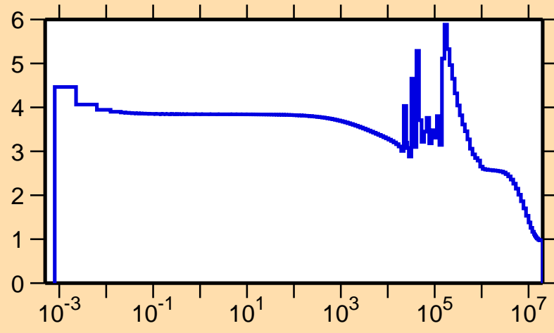
\sigma vs. E for ^{53}\text{Sc}(n,\text{el.})
