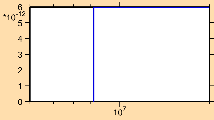
\sigma vs. E for ^{53}\text{Sc}(n,2np)
