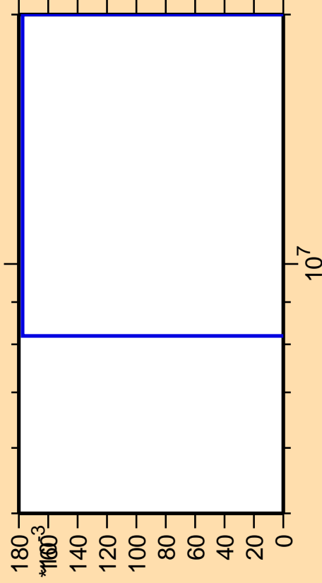
\Delta\sigma/\sigma vs. E for ^{53}\text{Sc}(n,2n\alpha)
