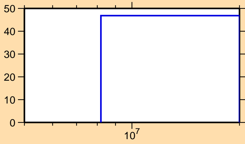
\Delta\sigma/\sigma vs. E for ^{53}\text{Sc}(n,\gamma)
