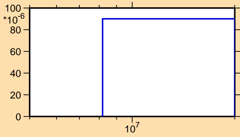
\sigma vs. E for ^{53}\text{Sc}(n,\alpha)
