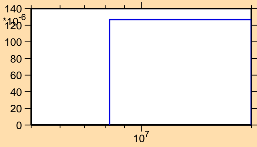
\sigma vs. E for ^{53}\text{Sc}(n,t)
