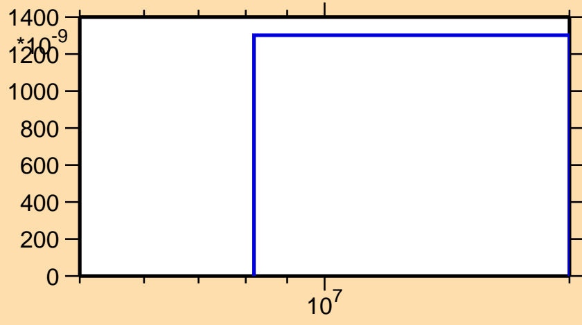
\sigma vs. E for ^{53}\text{Sc}(n,n\alpha)
