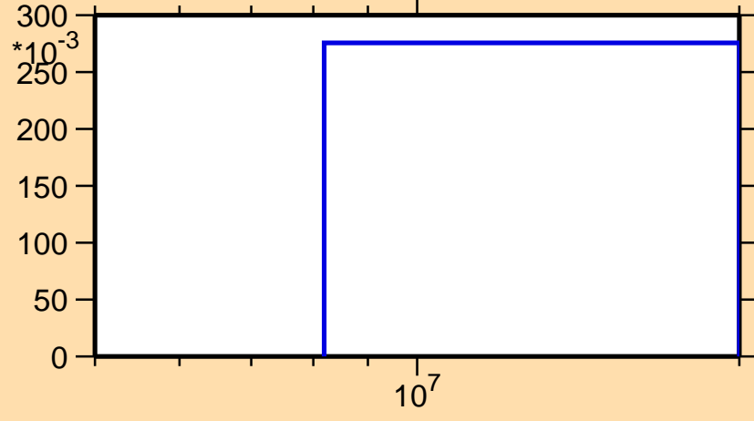
\sigma vs. E for ^{53}\text{Sc}(n,3n)
