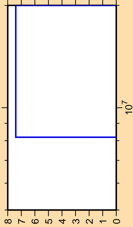
\Delta\sigma/\sigma vs. E for ^{53}\text{Sc}(n,2np)
