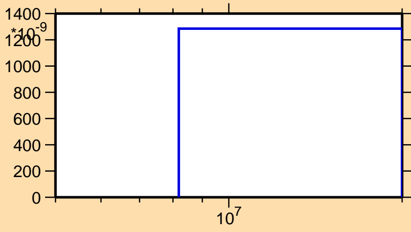
\sigma vs. E for ^{53}\text{Sc}(n,nt)
