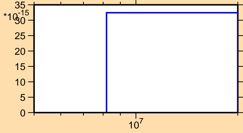
\sigma vs. E for ^{53}\text{Sc}(n,2n\alpha)
