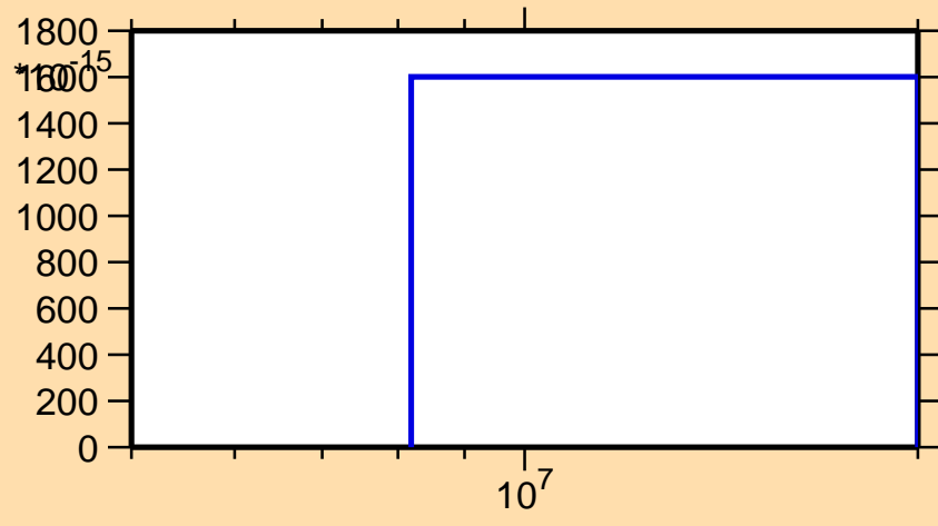
\sigma vs. E for ^{68}\text{Se}(\text{mt } 34)
