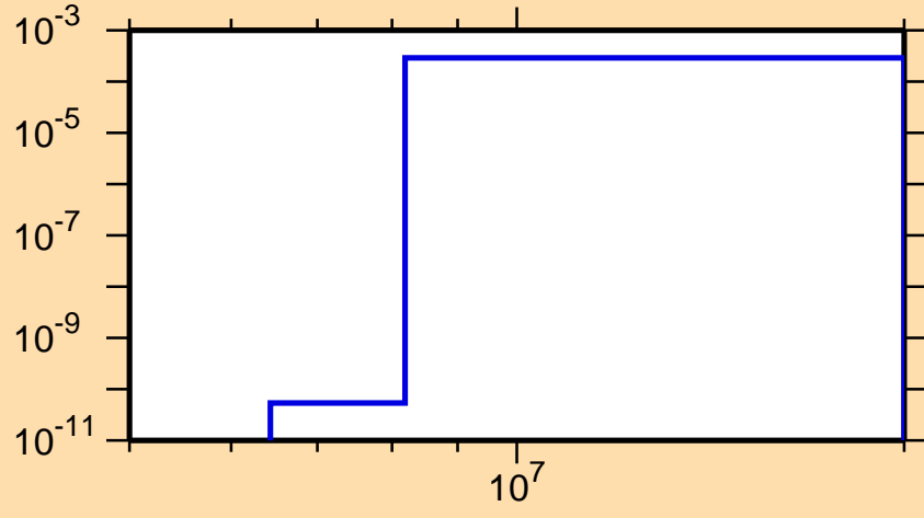
\sigma vs. E for ^{68}\text{Se}(n,\text{pd})
