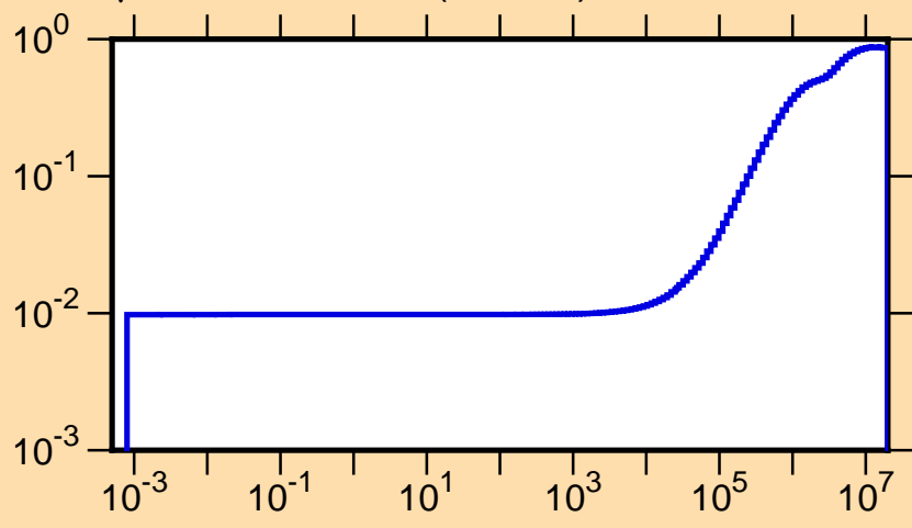
\mu vs. E for ^{69}\text{Se}(\text{mt251})
