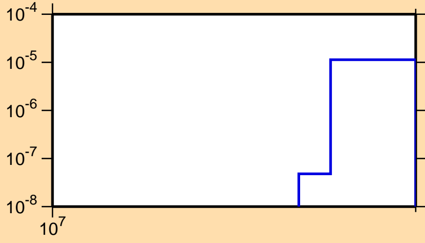
\sigma vs. E for ^{69}\text{Se}(n,2np)
