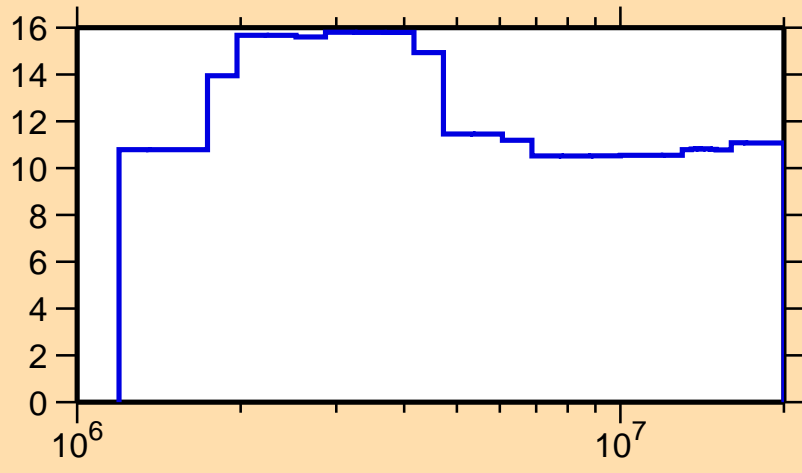
\Delta\sigma/\sigma vs. E for ^{69}\text{Se}(n,n\text{onel.})
