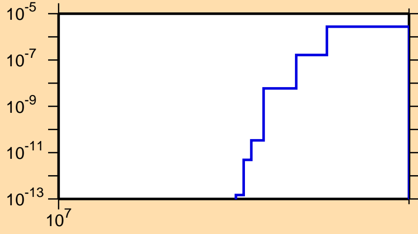
\sigma vs. E for ^{69}\text{Se}(n,\text{nd})
