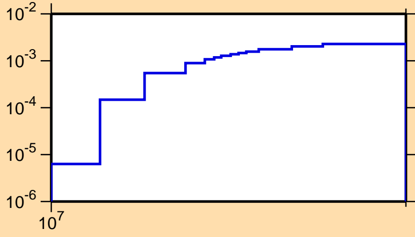
\sigma vs. E for ^{69}\text{Se}(n,2n)
