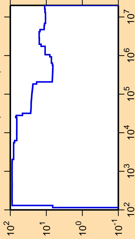
\Delta\sigma/\sigma vs. E for ^{69}\text{Se}(n,\text{nonel.})
