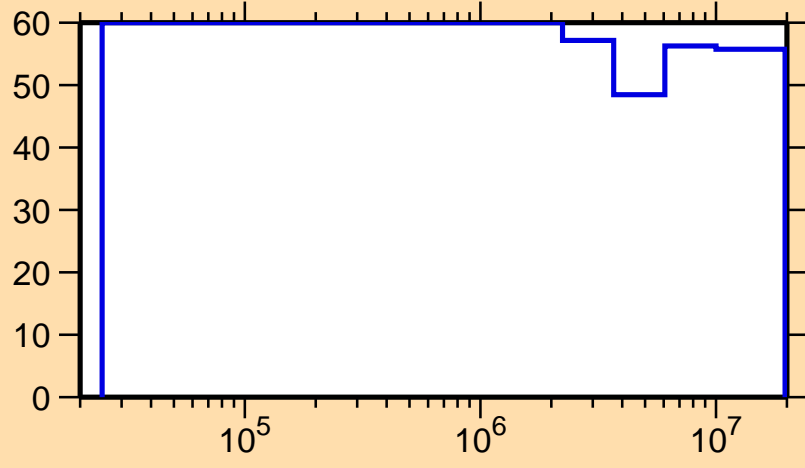
\Delta\sigma/\sigma vs. E for ^{69}\text{Se}(n,n_1)
