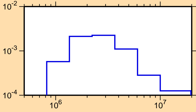
\sigma vs. E for ^{69}\text{Se}(n,n_4)
