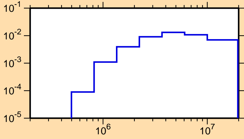
\sigma vs. E for ^{69}\text{Se}(n,n_3)
