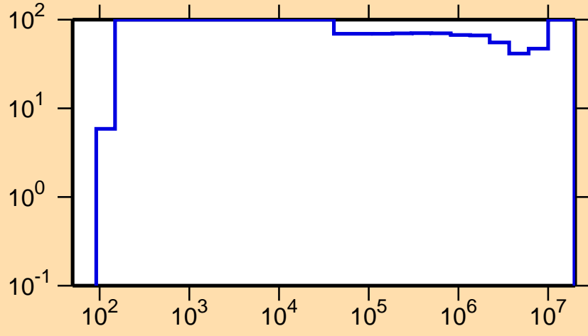
\Delta\sigma/\sigma vs. E for ^{69}\text{Se}(n,\gamma)
