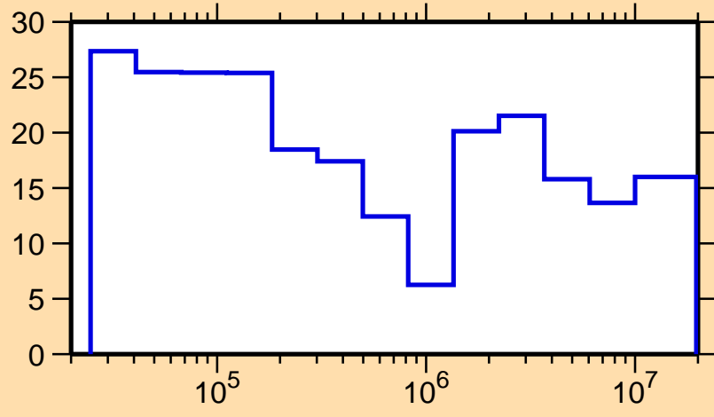
\Delta\sigma/\sigma vs. E for ^{69}\text{Se}(n,\text{el.})
