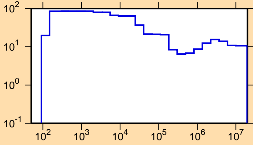
\Delta\sigma/\sigma vs. E for ^{69}\text{Se}(n,\text{nonel.})
