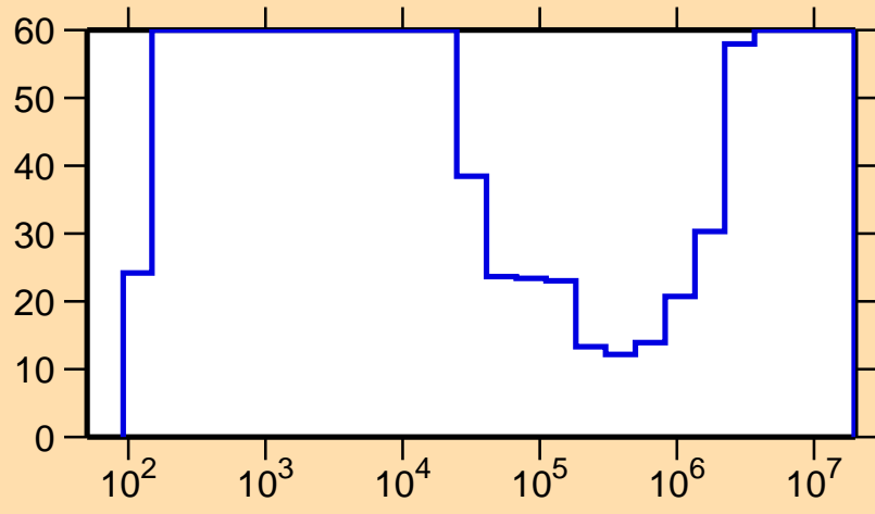
\Delta\sigma/\sigma vs. E for ^{69}\text{Se}(n,p)
