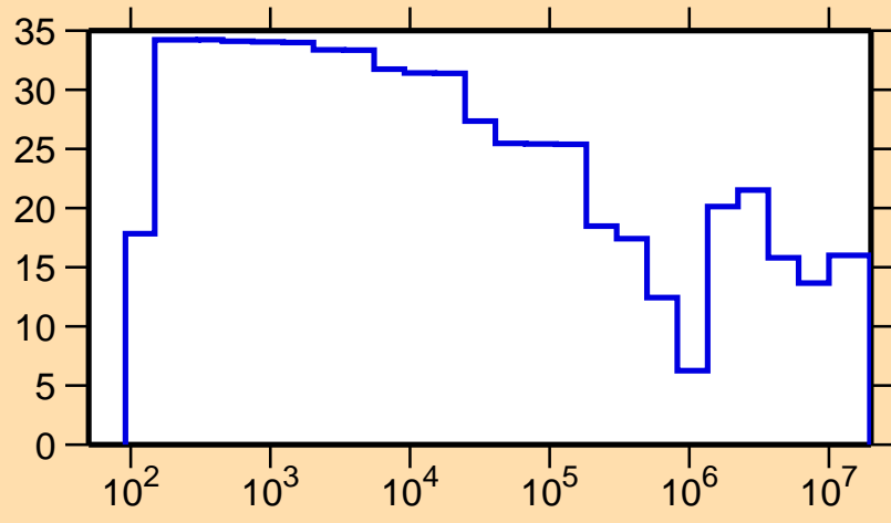
\Delta\sigma/\sigma vs. E for ^{69}\text{Se}(n,el.)
