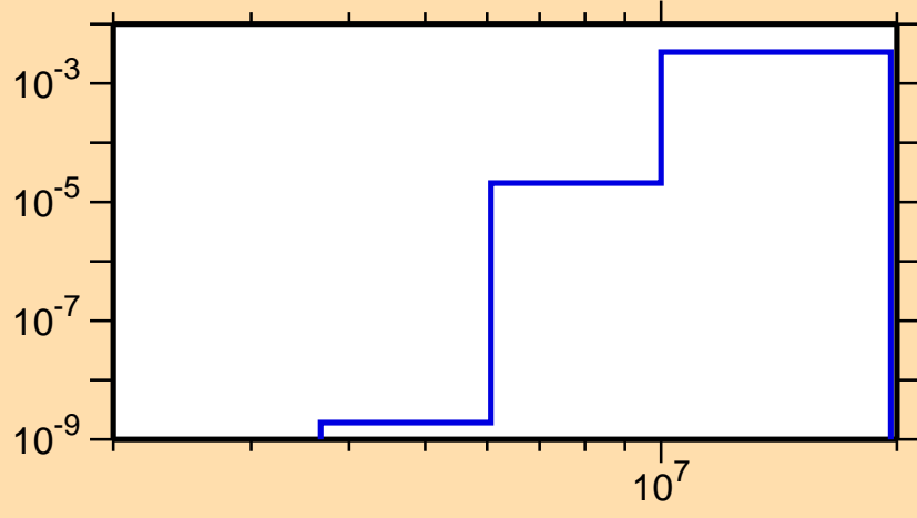
\sigma vs. E for ^{69}\text{Se}(n,n\alpha)
