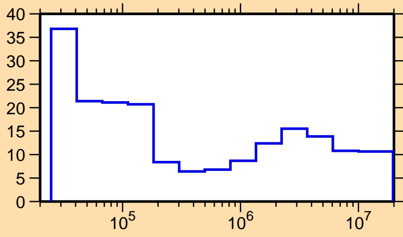
\Delta\sigma/\sigma vs. E for ^{69}\text{Se}(n,\text{nonel.})
