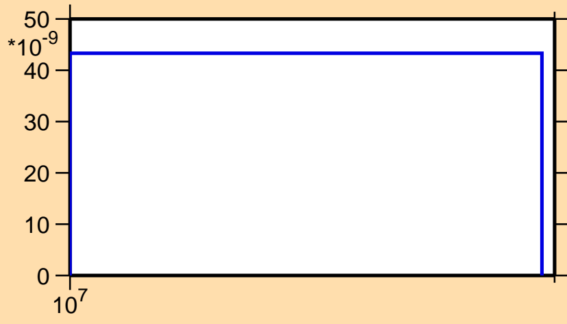
\sigma vs. E for ^{69}\text{Se} (mt 34)
