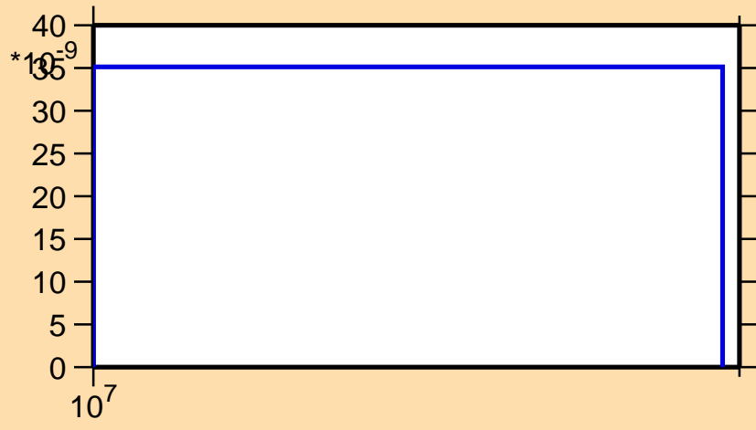
\sigma vs. E for ^{69}\text{Se}(n,nd)
