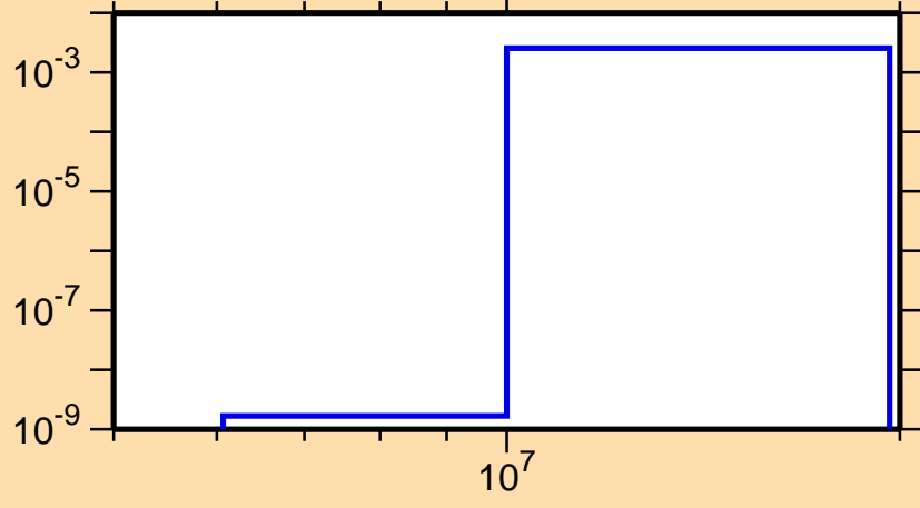
\sigma vs. E for ^{69}\text{Se}(n,\text{pd})
