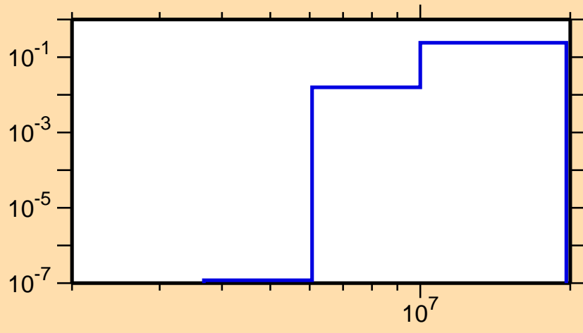
\sigma vs. E for ^{69}\text{Se}(n,np)
