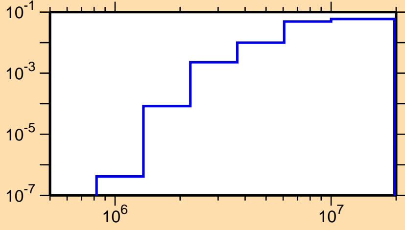
\sigma vs. E for ^{69}\text{Se}(n,n\text{cont.})
