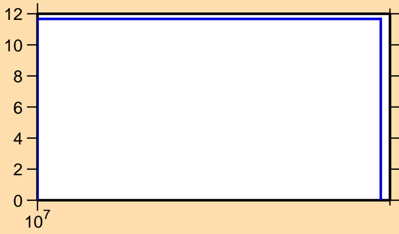
\Delta\sigma/\sigma vs. E for ^{69}\text{Se}(n,\text{tot.})
