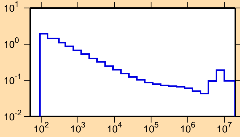
\sigma vs. E for ^{69}\text{Se}(n,\alpha)
