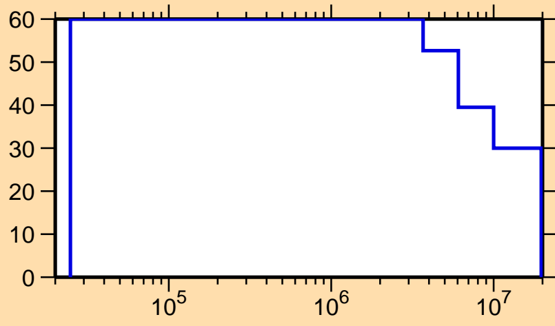
\Delta\sigma/\sigma vs. E for ^{69}\text{Se}(n,\text{inel.})
