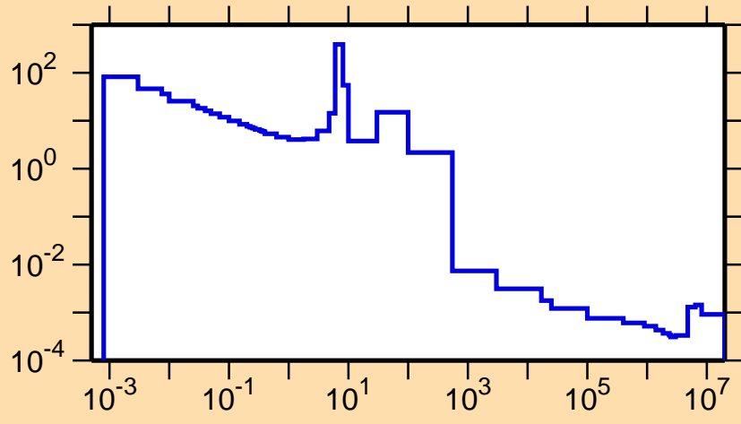
\sigma vs. E for ^{69}\text{Se}(n,\gamma)
