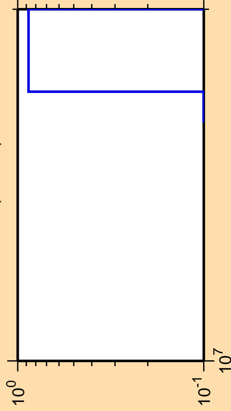
\Delta\sigma/\sigma vs. E for ^{70}\text{Se}(n,2n\alpha)
