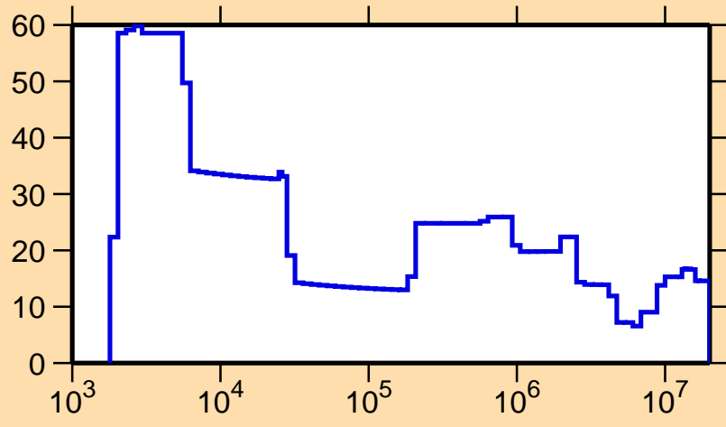
\Delta\sigma/\sigma vs. E for ^{70}\text{Se}(n,el.)
