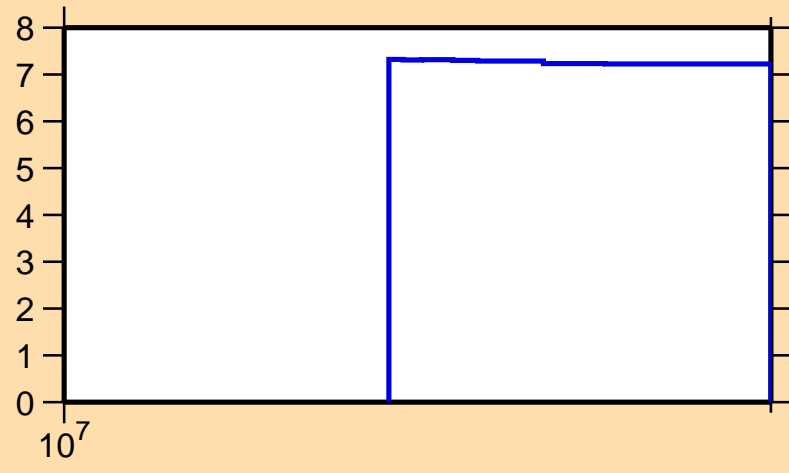
\Delta\sigma/\sigma vs. E for ^{70}\text{Se}(n,\text{nonel.})
