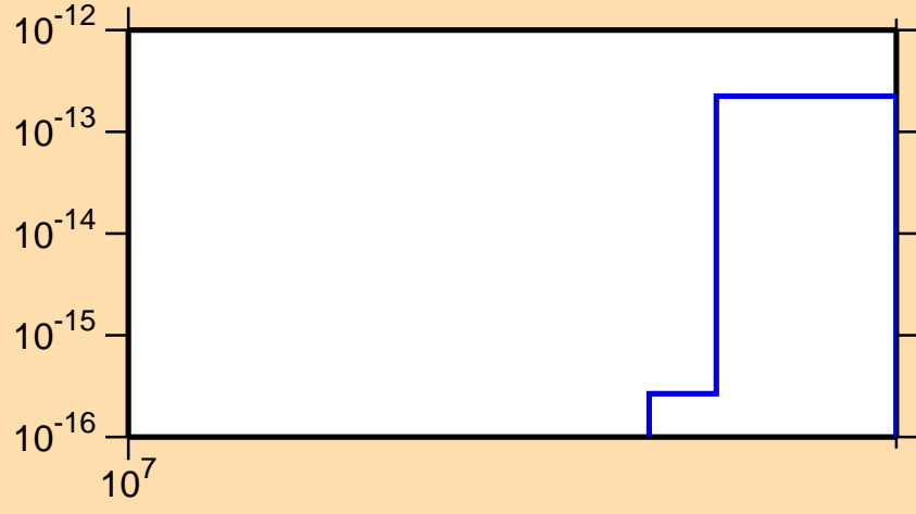
\sigma vs. E for ^{70}\text{Se}(n,2n\alpha)
