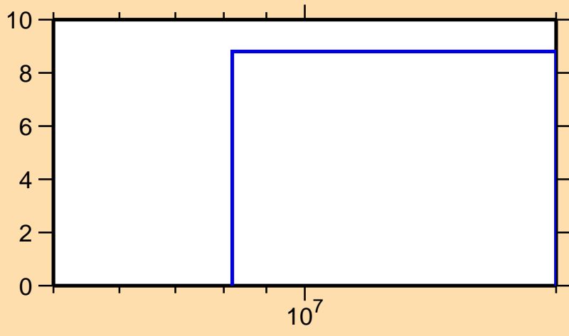
\Delta\sigma/\sigma vs. E for ^{70}\text{Se}(n,\text{tot.})
