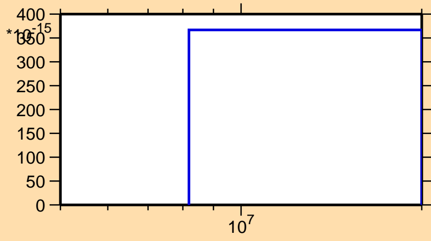
\sigma vs. E for ^{70}\text{Se} (mt 34)
