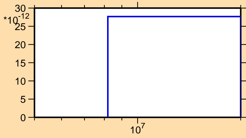
\sigma vs. E for ^{70}\text{Se}(n,\text{nd})
