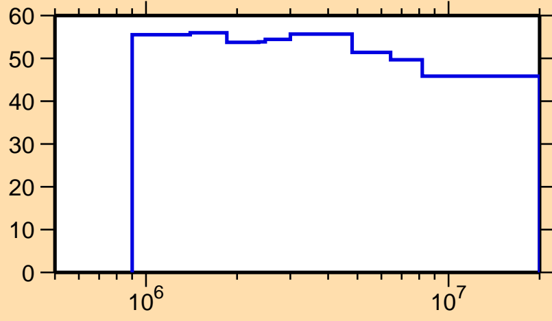
\Delta\sigma/\sigma vs. E for ^{70}\text{Se}(n,n_1)
