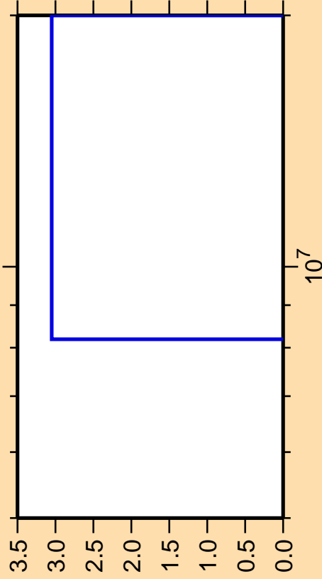
\Delta\sigma/\sigma vs. E for ^{70}\text{Se} (mt 34)
