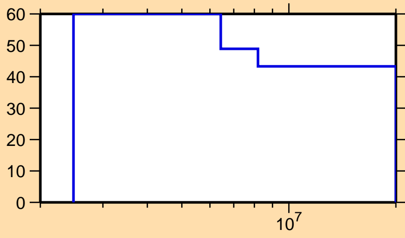
\Delta\sigma/\sigma vs. E for ^{70}\text{Se}(n,n\text{cont.})
