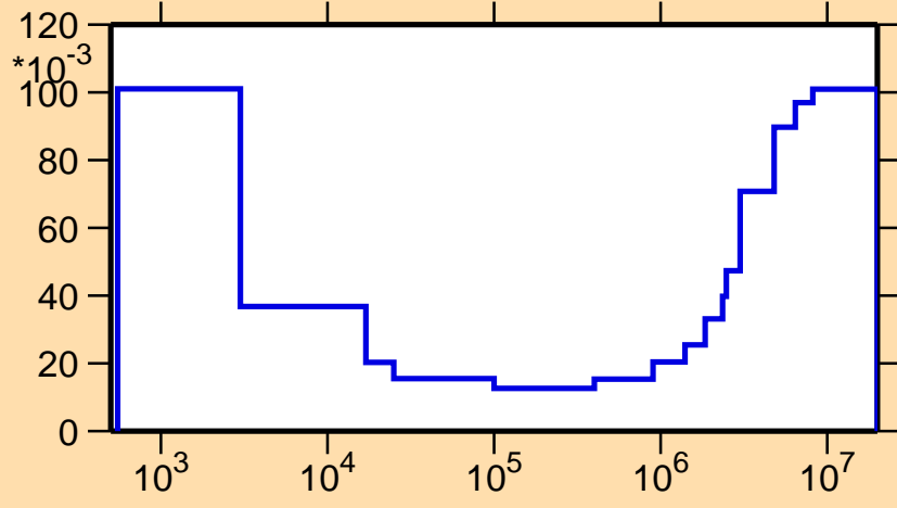
\sigma vs. E for ^{70}\text{Se}(n,\alpha)
