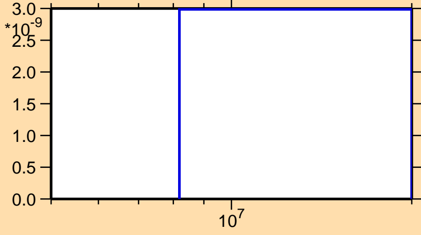
\sigma vs. E for ^{70}\text{Se}(n,\text{pt})
