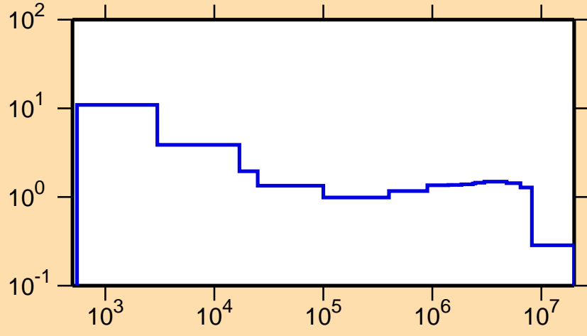
\sigma vs. E for ^{70}\text{Se}(n,p)
