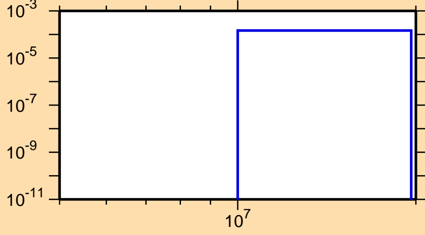
\sigma vs. E for ^{71}\text{Se}(n,pd)
