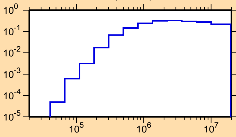
\sigma vs. E for ^{71}\text{Se}(n,\text{inel.})
