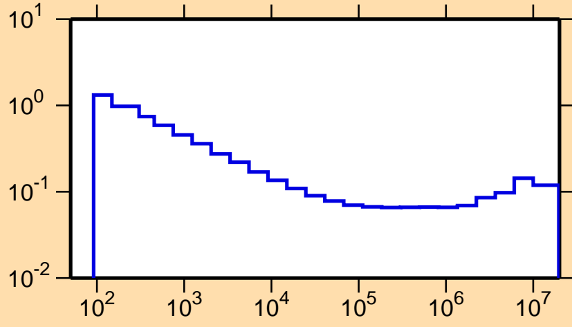
\sigma vs. E for ^{71}\text{Se}(n,\alpha)
