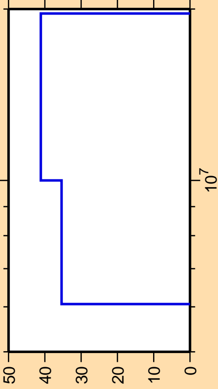
\Delta\sigma/\sigma vs. E for ^{71}\text{Se}(n,p)
