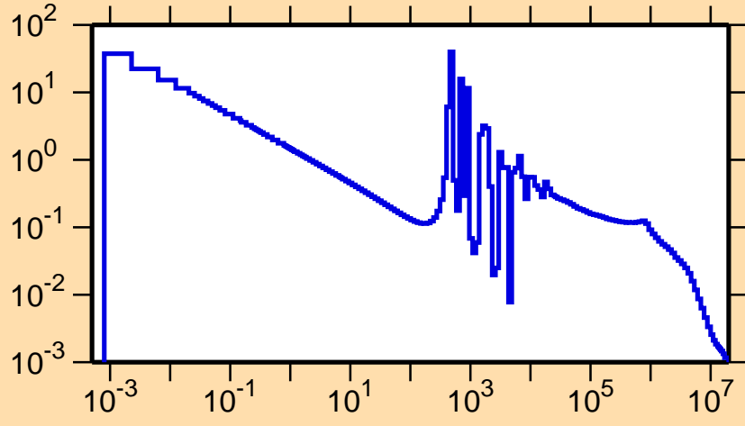
\sigma vs. E for ^{72}\text{Se}(n,\gamma)
