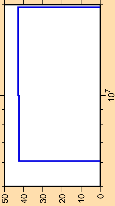
\Delta\sigma/\sigma vs. E for ^{72}\text{Se}(n,np)
