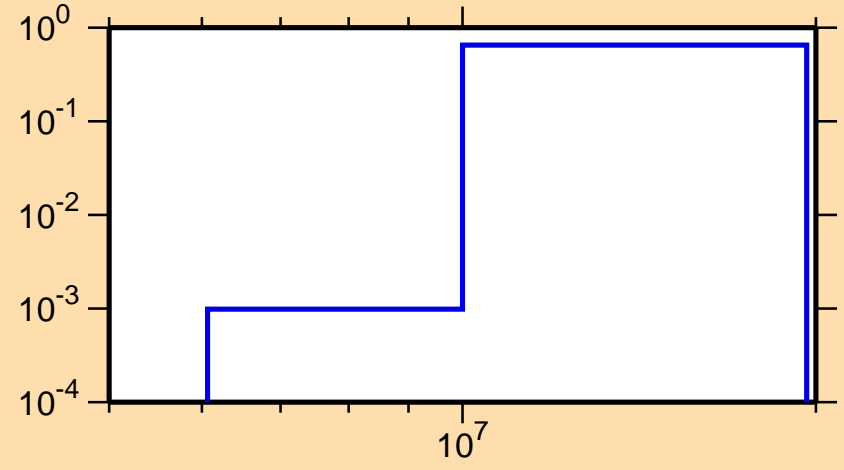
\sigma vs. E for ^{72}\text{Se}(n,np)
