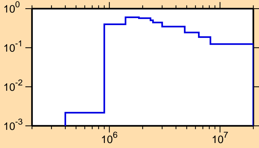
\sigma vs. E for ^{72}\text{Se}(n,n_1)
