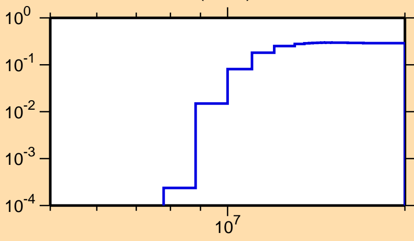
\sigma vs. E for ^{73}\text{Se}(n,2n)
