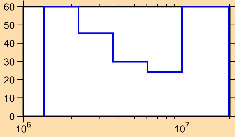
\Delta\sigma/\sigma vs. E for ^{73}\text{Se}(n,n\text{cont.})
