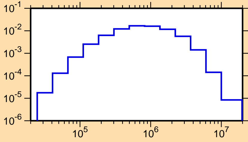
\sigma vs. E for ^{73}\text{Se}(n,n_1)
