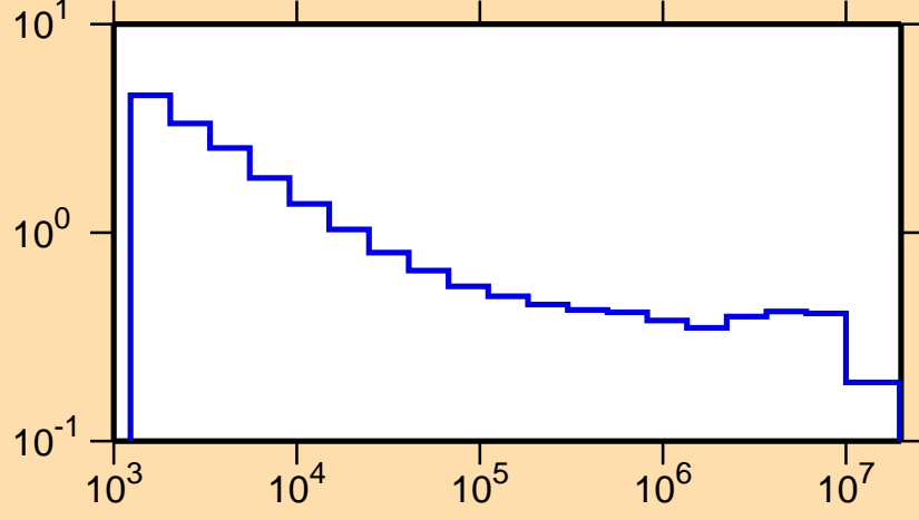
\sigma vs. E for ^{73}\text{Se}(n,p)
