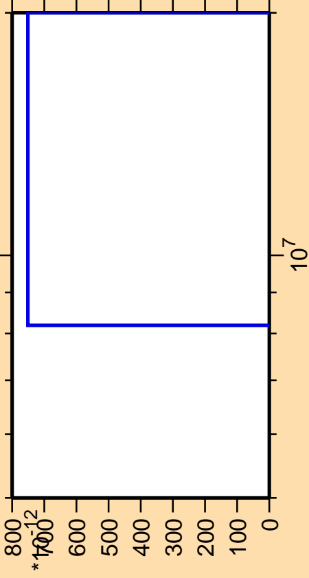
\Delta\sigma/\sigma vs. E for ^{73}\text{Se}(n,nt)
