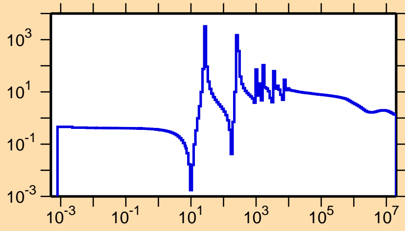
\sigma vs. E for ^{74}\text{Se}(n,\text{el.})
