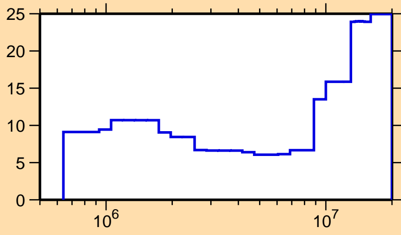
\Delta\sigma/\sigma vs. E for ^{74}\text{Se}(n,\text{inel.})
