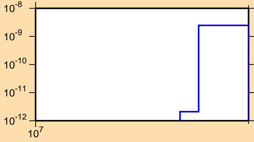
\sigma vs. E for ^{74}\text{Se}(\text{mt117})
