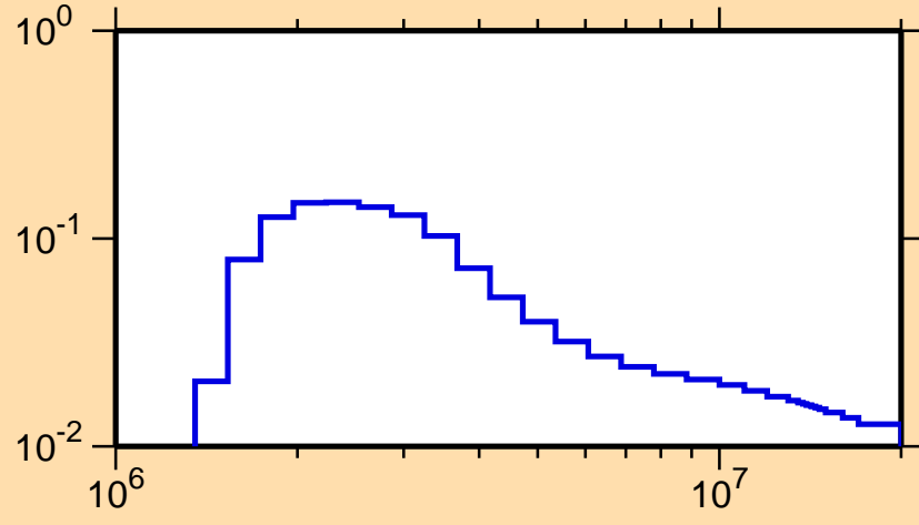
\sigma vs. E for ^{74}\text{Se}(n,n_4)
