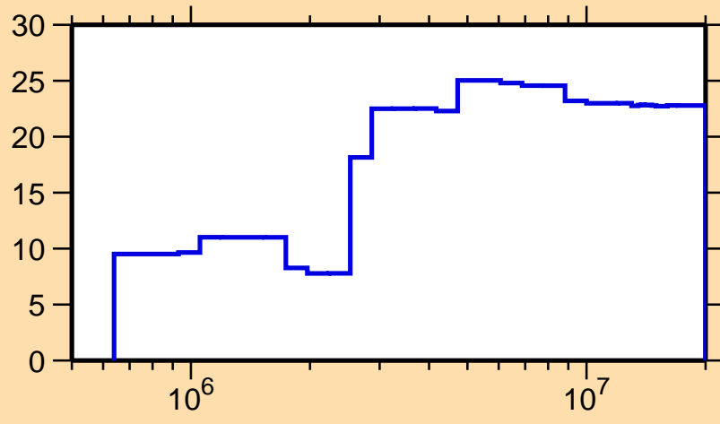
\Delta\sigma/\sigma vs. E for ^{74}\text{Se}(n,n_1)
