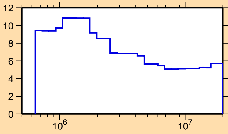
\Delta\sigma/\sigma vs. E for ^{74}\text{Se}(n,\text{nonel.})
