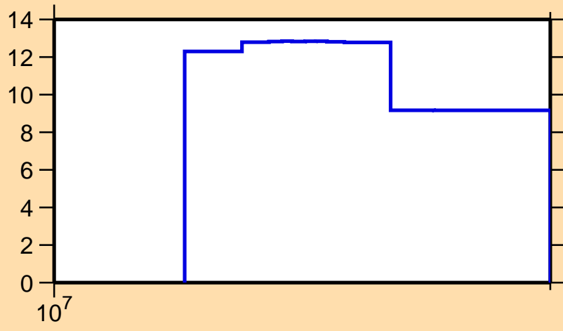
\Delta\sigma/\sigma vs. E for ^{74}\text{Se}(n,\text{el.})
