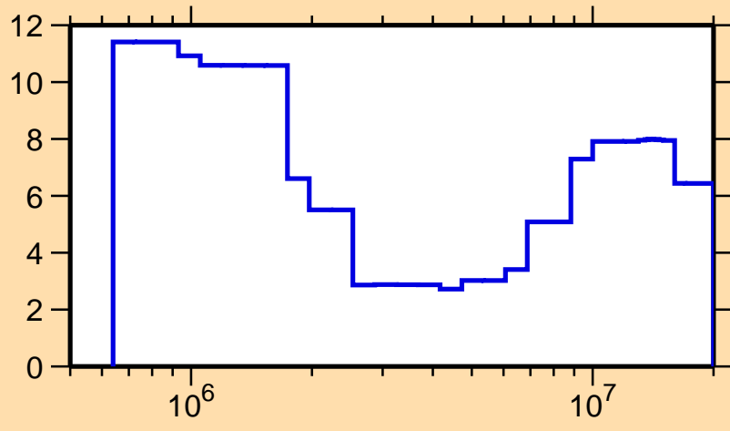
\Delta\sigma/\sigma vs. E for ^{74}\text{Se}(n,\text{tot.})
