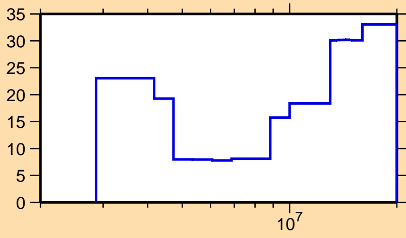
\Delta\sigma/\sigma vs. E for ^{74}\text{Se}(n,n\text{cont.})
