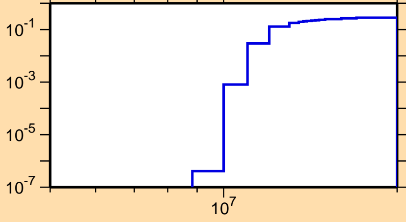
\sigma vs. E for ^{74}\text{Se}(n,np)
