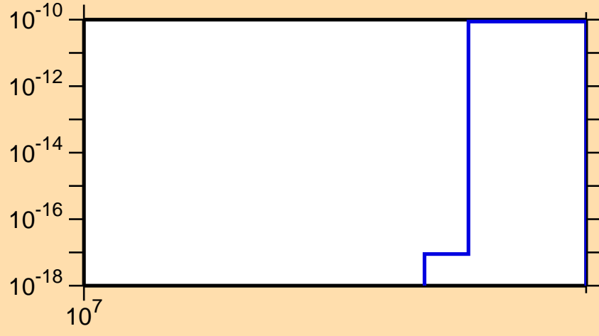
\sigma vs. E for ^{74}\text{Se}(n,2n\alpha)
