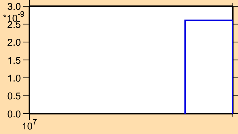
\sigma vs. E for ^{74}\text{Se}(n,\text{nd})
