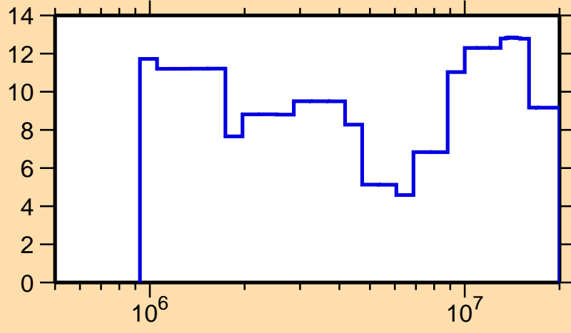
\Delta\sigma/\sigma vs. E for ^{74}\text{Se}(n,el.)
