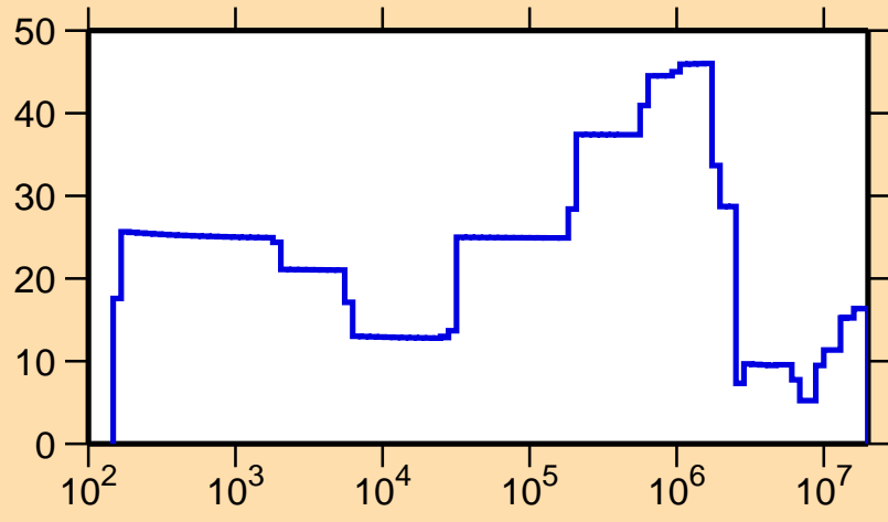
\Delta\sigma/\sigma vs. E for ^{75}\text{Se}(n,el.)
