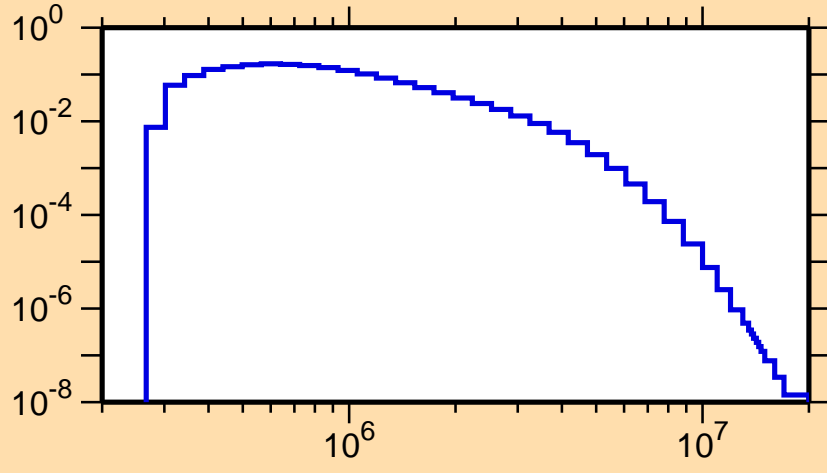
\sigma vs. E for ^{75}\text{Se}(n,n_3)
