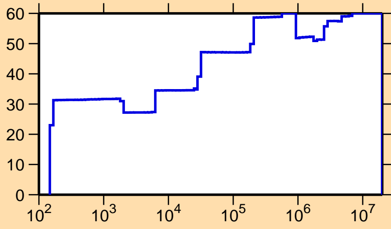
\Delta\sigma/\sigma vs. E for ^{75}\text{Se}(n,\gamma)
