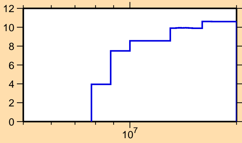
\Delta\sigma/\sigma vs. E for ^{75}\text{Se}(n,\text{tot.})
