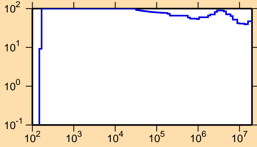
\Delta\sigma/\sigma vs. E for ^{75}\text{Se}(n,p)
