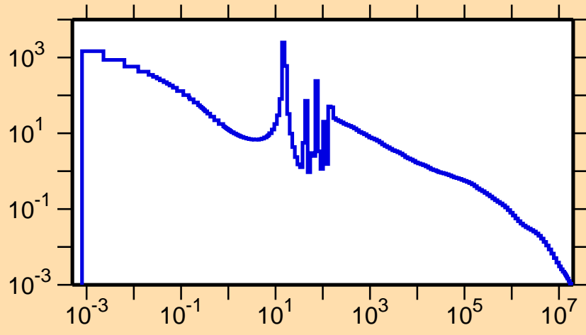
\sigma vs. E for ^{75}\text{Se}(n,\gamma)
