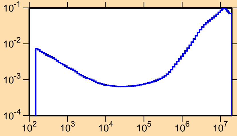
\sigma vs. E for ^{75}\text{Se}(n,p)
