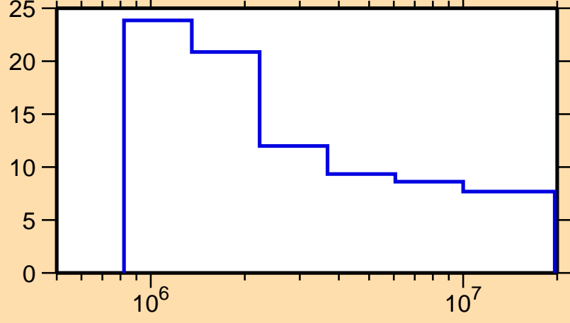
\Delta\sigma/\sigma vs. E for ^{75}\text{Se}(n,n\text{onel.})
