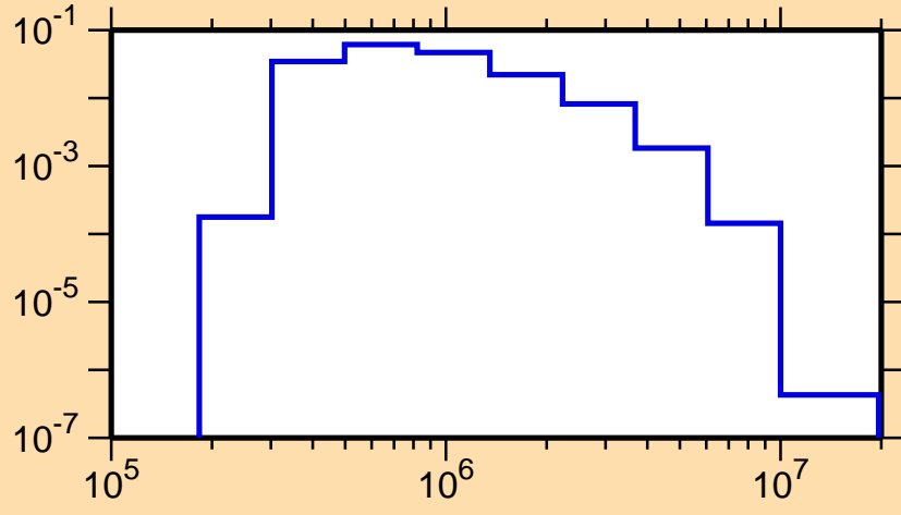
\sigma vs. E for ^{75}\text{Se}(n,n_4)
