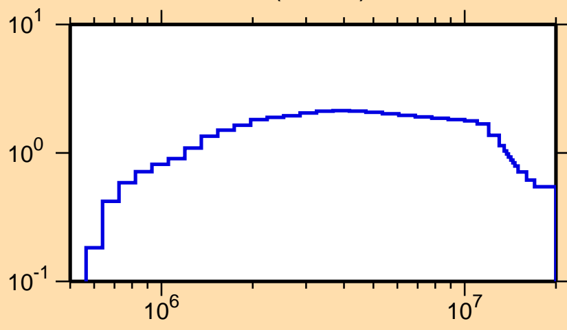
\sigma vs. E for ^{76}\text{Se}(n,\text{inel.})
