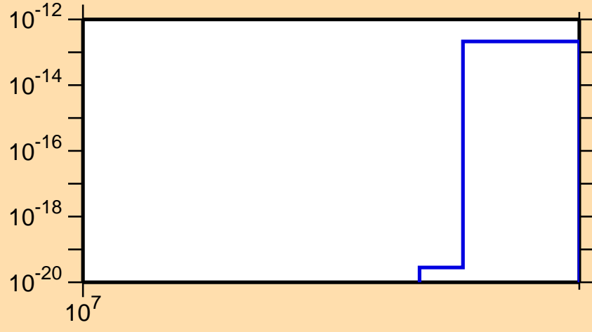
\sigma vs. E for ^{76}\text{Se}(\text{mt117})
