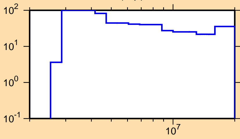
\Delta\sigma/\sigma vs. E for ^{76}\text{Se}(n,p)
