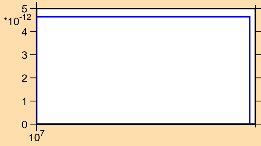
\sigma vs. E for ^{76}\text{Se}(n,\text{nd})
