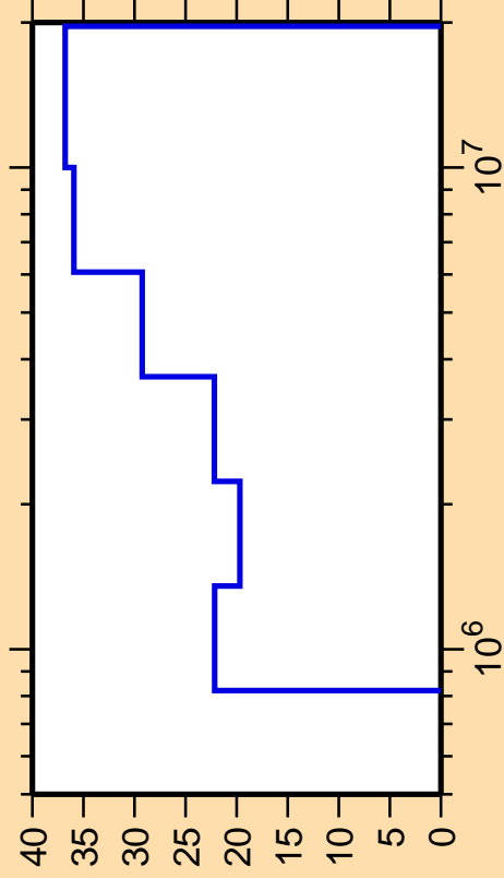
\Delta\sigma/\sigma vs. E for ^{76}\text{Se}(n,n_4)
