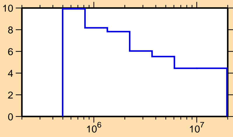
\Delta\sigma/\sigma vs. E for ^{76}\text{Se}(n,\text{nonel.})
