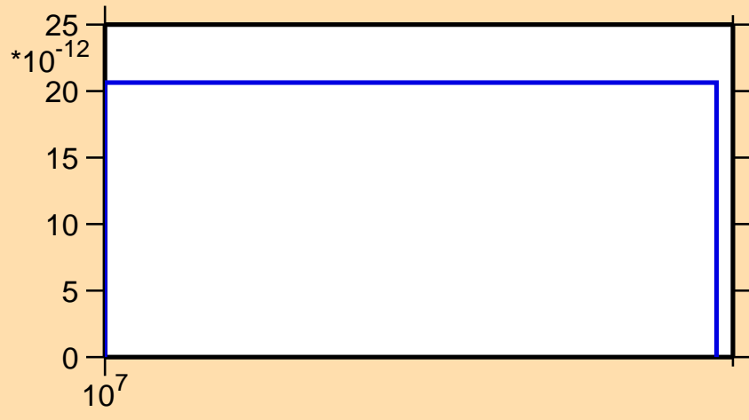
\sigma vs. E for ^{76}\text{Se}(n,pd)
