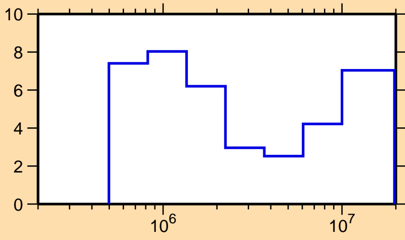
\Delta\sigma/\sigma vs. E for ^{76}\text{Se}(n,\text{tot.})
