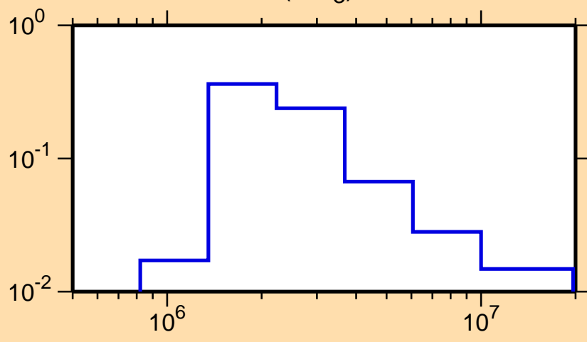
\sigma vs. E for ^{76}\text{Se}(n,n_3)
