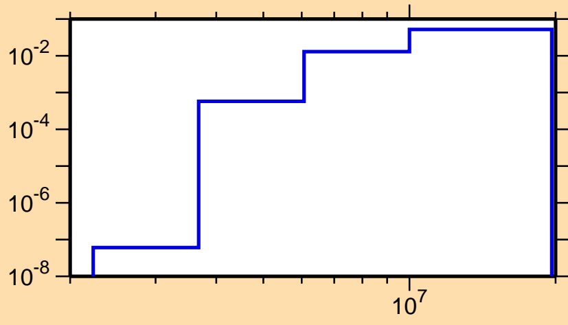
\sigma vs. E for ^{76}\text{Se}(n,p)
