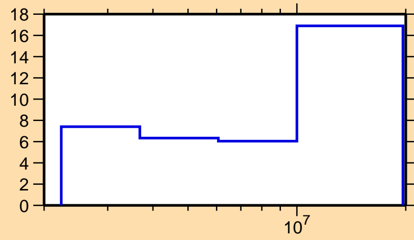
\Delta\sigma/\sigma vs. E for ^{76}\text{Se}(n,n\text{cont.})
