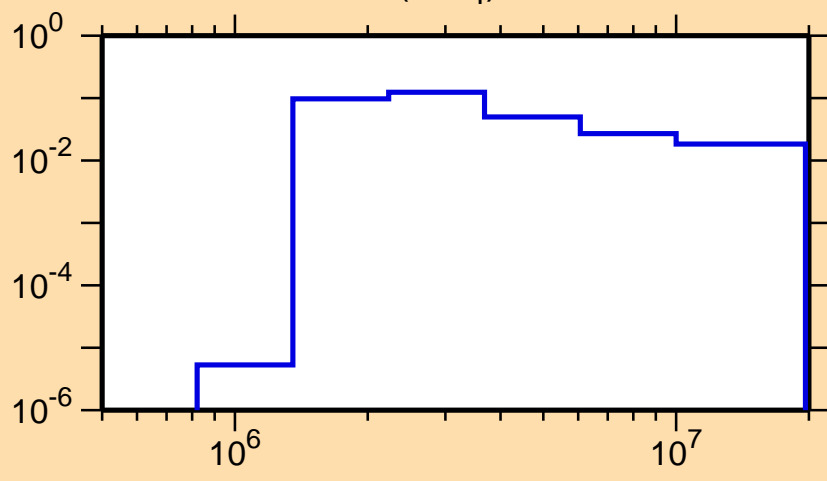
\sigma vs. E for ^{76}\text{Se}(n,n_4)
