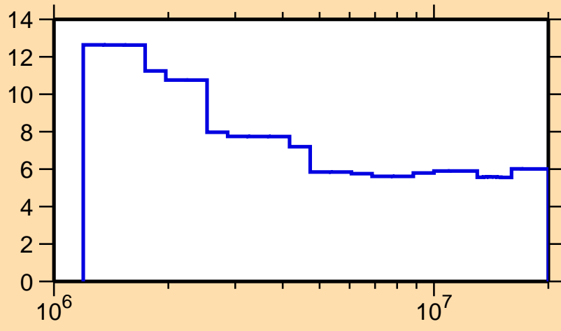
\Delta\sigma/\sigma vs. E for ^{77}\text{Se}(n,n\text{onrel.})
