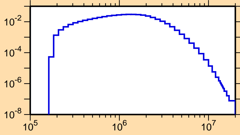
\sigma vs. E for ^{77}\text{Se}(n,n_2)
