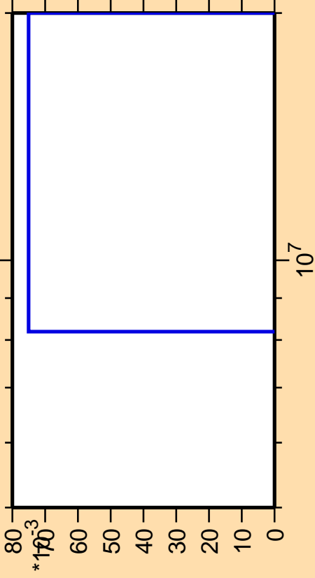
\Delta\sigma/\sigma vs. E for ^{77}\text{Se}(n,\text{pt})
