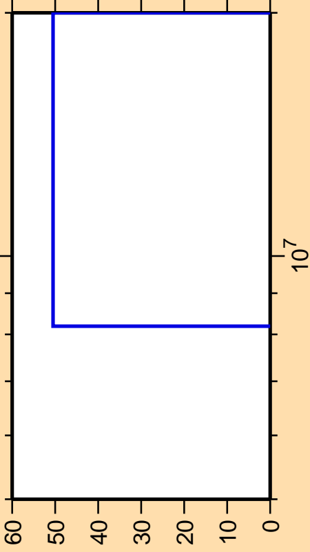
\Delta\sigma/\sigma vs. E for ^{77}\text{Se}(n,np)
