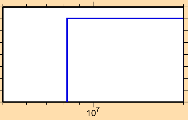
\sigma vs. E for ^{77}\text{Se}(n,\text{pt})
