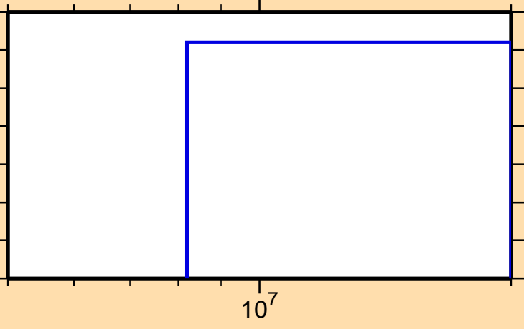
\sigma vs. E for ^{77}\text{Se}(n,\text{pt})
