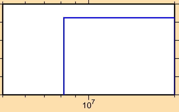
\sigma vs. E for ^{77}\text{Se}(n,\text{nd})
