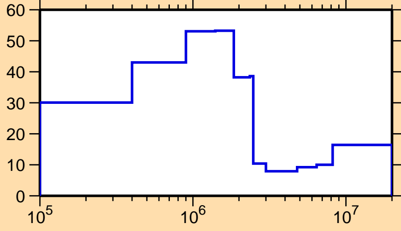
\Delta\sigma/\sigma vs. E for ^{77}\text{Se}(n,el.)
