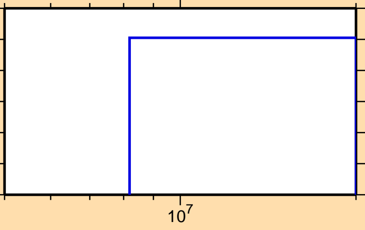
\sigma vs. E for ^{77}\text{Se}(n,2n\alpha)
