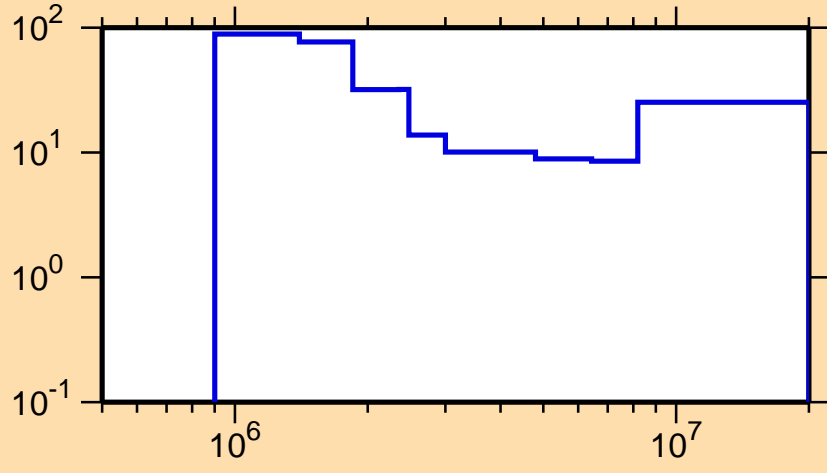
\Delta\sigma/\sigma vs. E for ^{79}\text{Se}(n,n\text{cont.})
