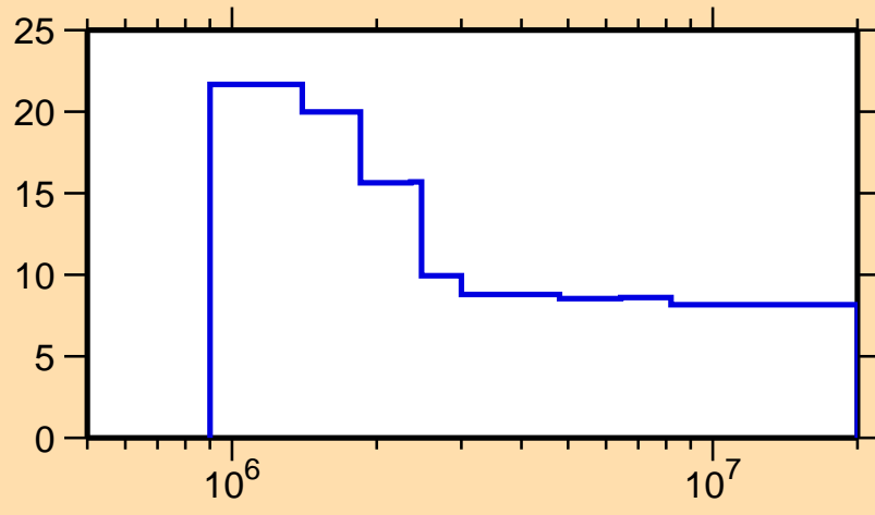
\Delta\sigma/\sigma vs. E for ^{79}\text{Se}(n,n\text{onrel.})
