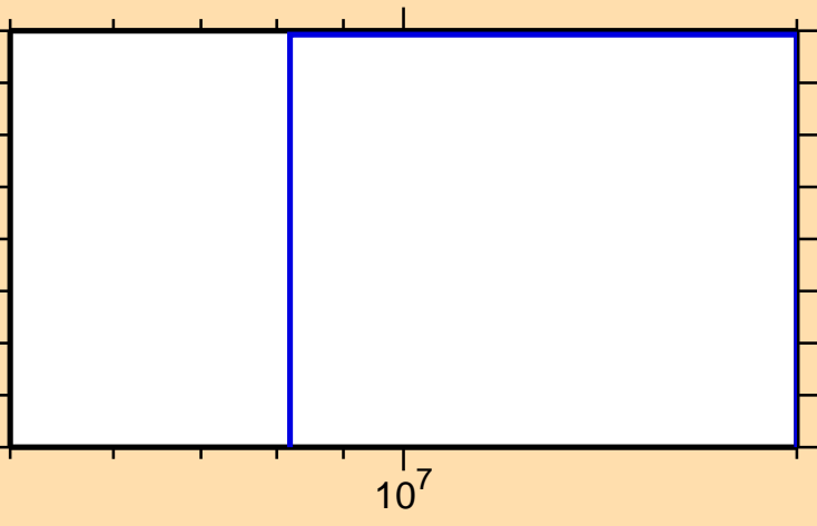
\sigma vs. E for ^{79}\text{Se}(n,d)
