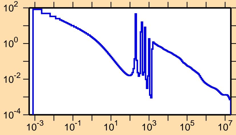
\sigma vs. E for ^{79}\text{Se}(n,\gamma)
