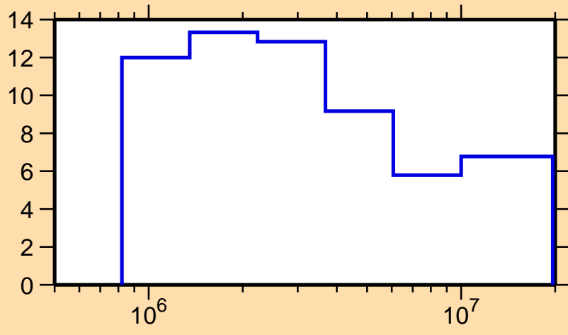
\Delta\sigma/\sigma vs. E for ^{79}\text{Se}(n,n\text{onel.})
