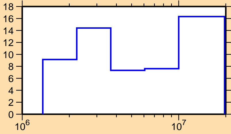
\Delta\sigma/\sigma vs. E for ^{79}\text{Se}(n,el.)
