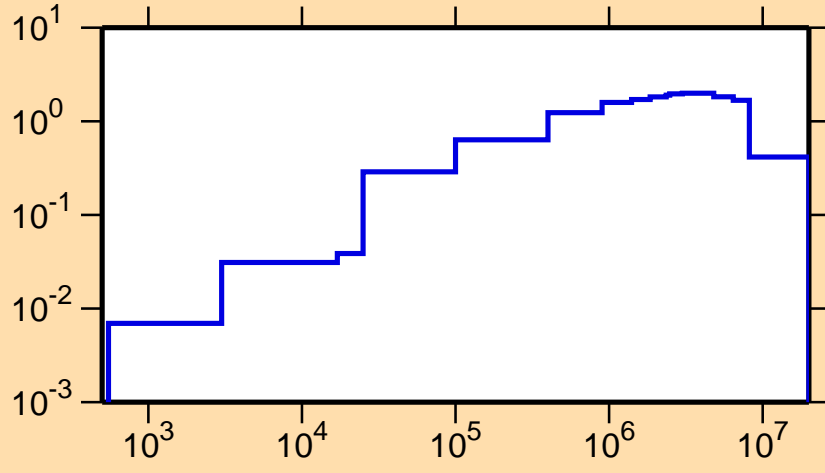
\sigma vs. E for ^{79}\text{Se}(n,\text{inel.})
