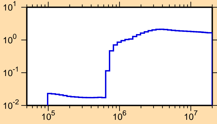
\sigma vs. E for ^{80}\text{Se}(n,\text{nonel.})
