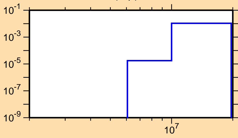
\sigma vs. E for ^{80}\text{Se}(n,p)
