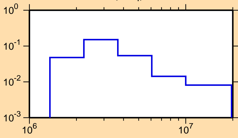
\sigma vs. E for ^{80}\text{Se}(n,n_4)
