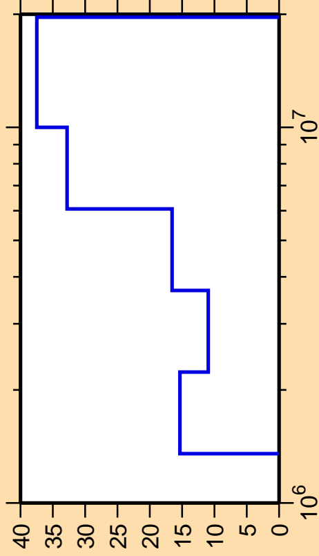
\Delta\sigma/\sigma vs. E for ^{80}\text{Se}(n,n_4)
