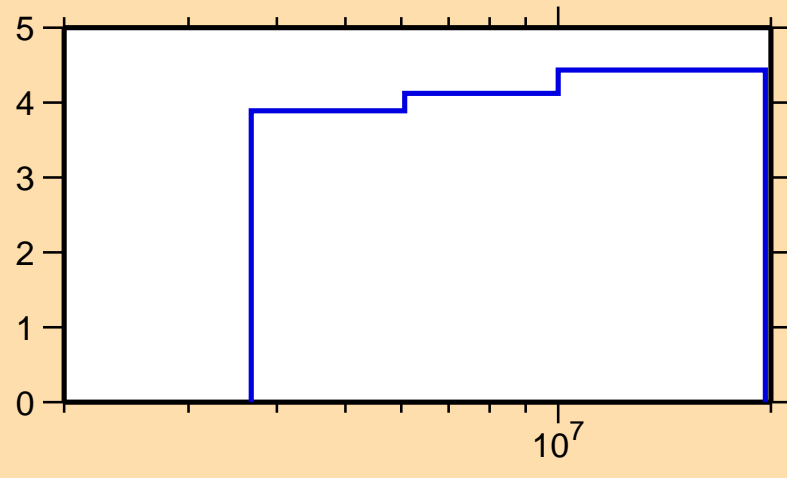
\Delta\sigma/\sigma vs. E for ^{80}\text{Se}(n,\text{nonel.})
