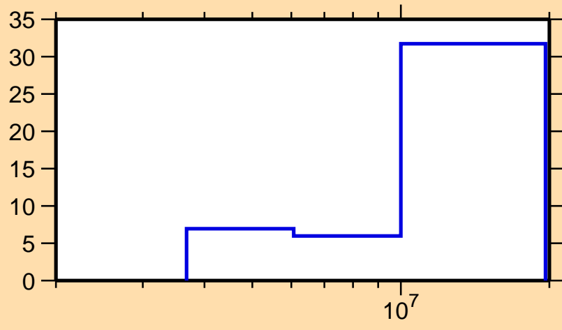
\Delta\sigma/\sigma vs. E for ^{80}\text{Se}(n,ncont.)
