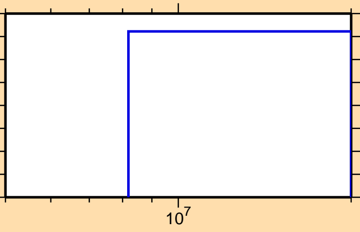
\sigma vs. E for ^{80}\text{Se}(n,np)
