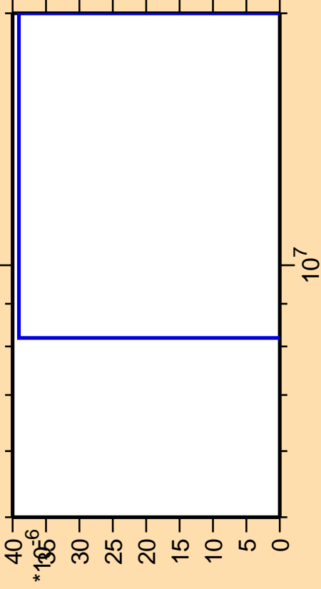
\Delta\sigma/\sigma vs. E for ^{80}\text{Se}(n,2n\alpha)
