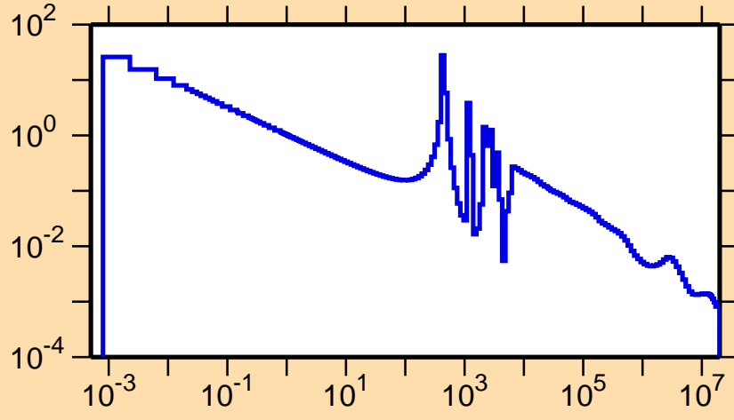
\sigma vs. E for ^{81}\text{Se}(n,\gamma)
