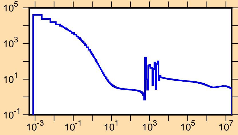
\sigma vs. E for ^{81}\text{Se}(n,\text{tot.})
