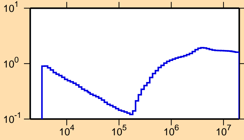
\sigma vs. E for ^{81}\text{Se}(n,\text{nonel.})
