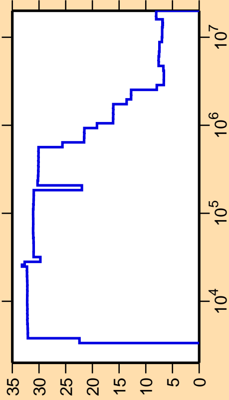
\Delta\sigma/\sigma vs. E for ^{81}\text{Se}(n,\text{nonel.})
