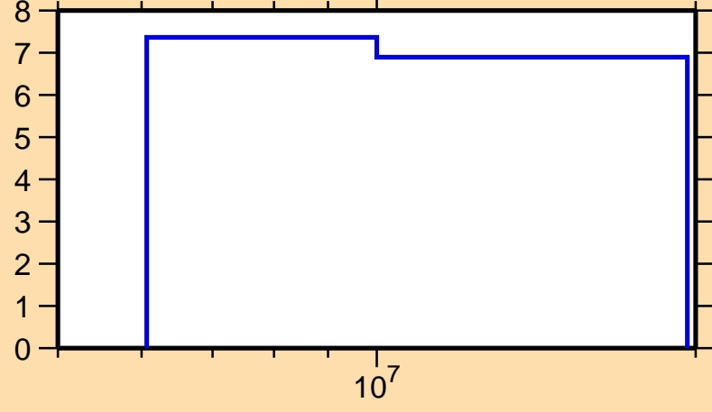
\Delta\sigma/\sigma vs. E for ^{81}\text{Se}(n,\text{nonel.})
