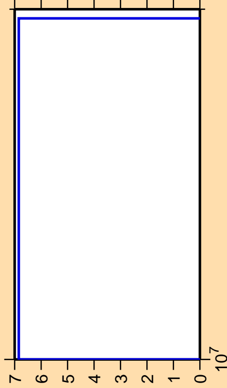
\Delta\sigma/\sigma vs. E for ^{81}\text{Se}(n,2n\alpha)
