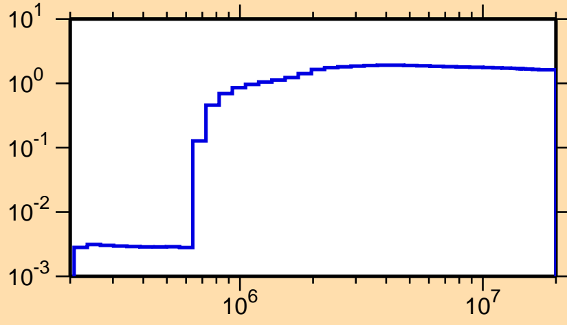
\sigma vs. E for ^{82}\text{Se}(n,\text{nonel.})
