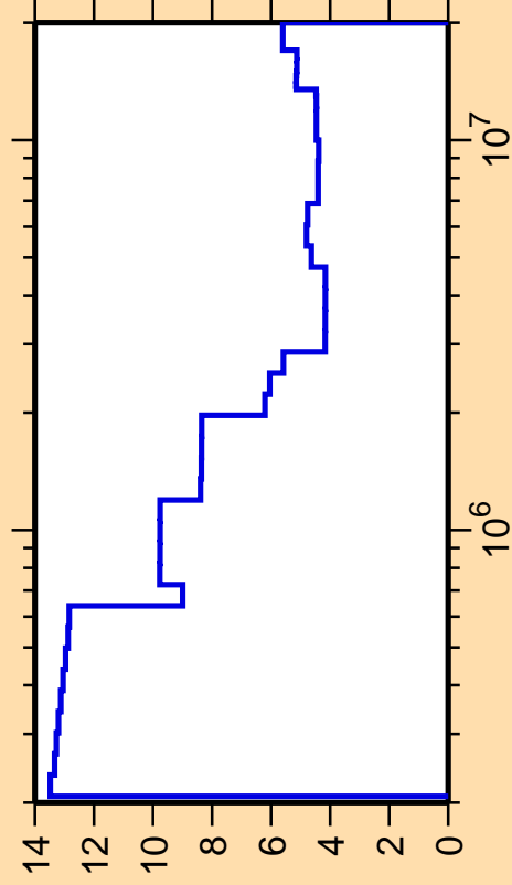
\Delta\sigma/\sigma vs. E for ^{82}\text{Se}(n,\text{nonel.})
