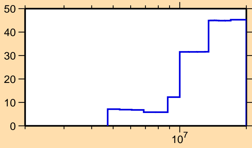
\Delta\sigma/\sigma vs. E for ^{82}\text{Se}(n,n\text{cont.})
