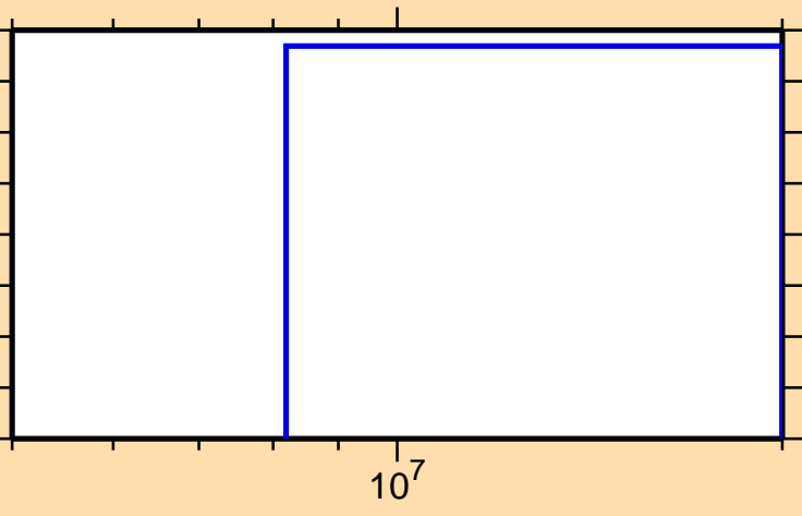
\sigma vs. E for ^{82}\text{Se}(n,np)
