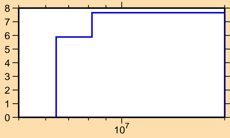
\Delta\sigma/\sigma vs. E for ^{82}\text{Se}(n,el.)
