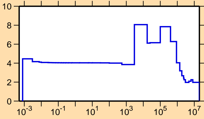
\sigma vs. E for ^{82}\text{Se}(n,\text{el.})
