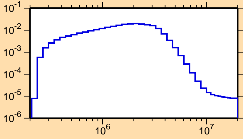
\sigma vs. E for ^{83}\text{Se}(n,n_1)
